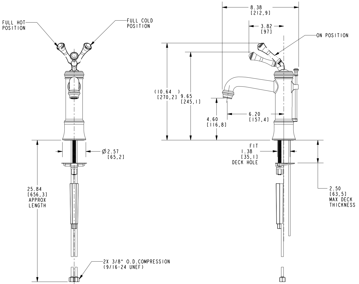
SINGLE HOLE LAVATORY FAUCET
