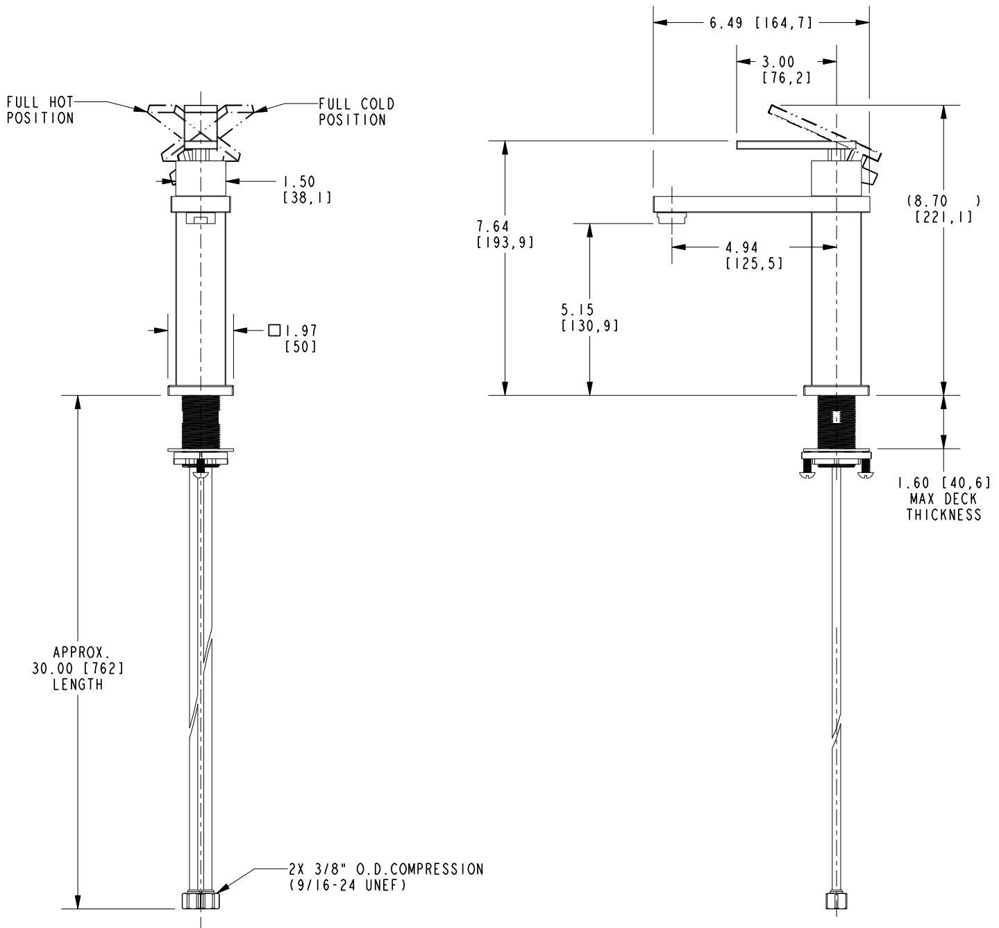
SINGLE HOLE LAVATORY FAUCET
