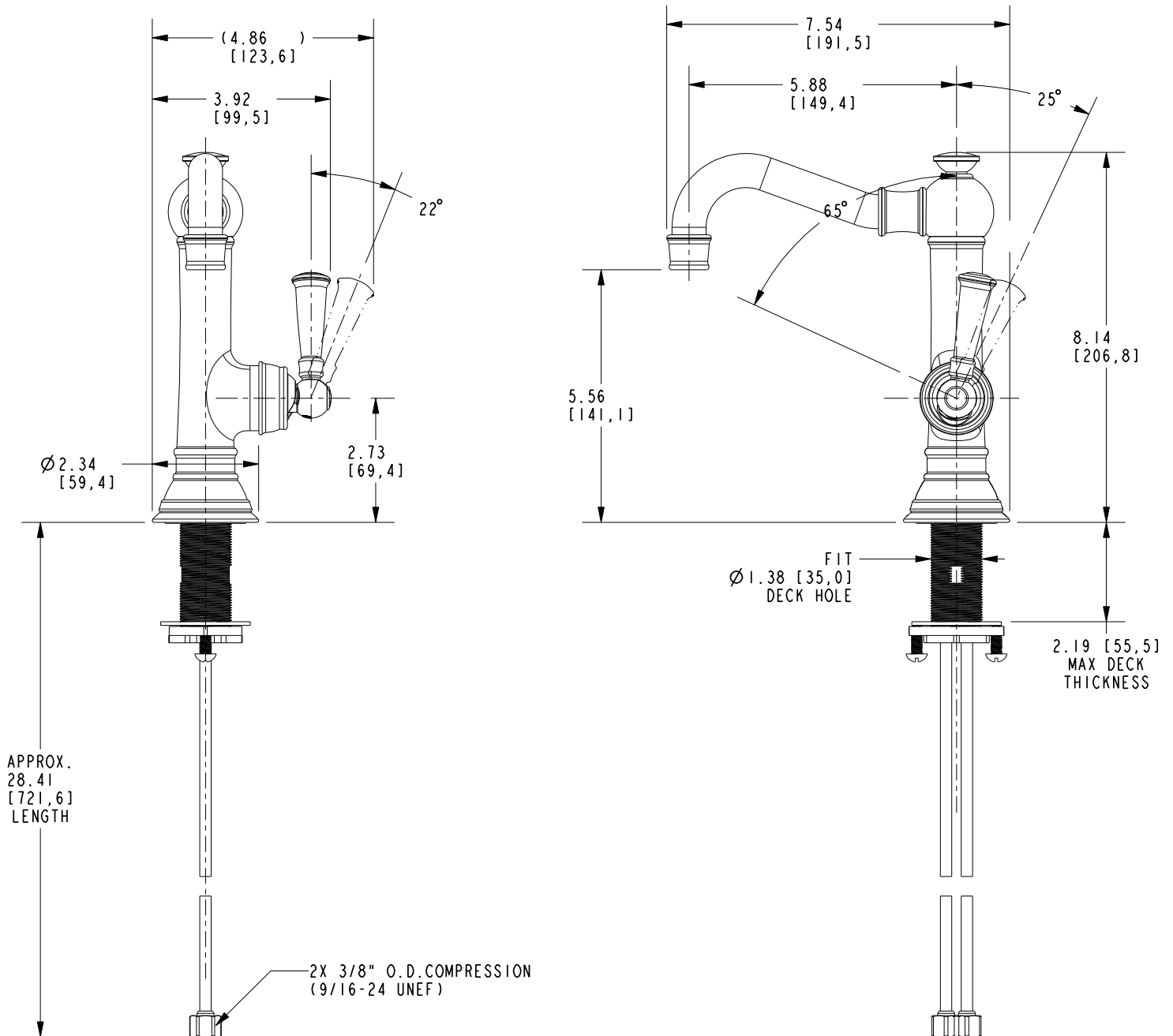
SINGLE HOLE LAVATORY FAUCET
