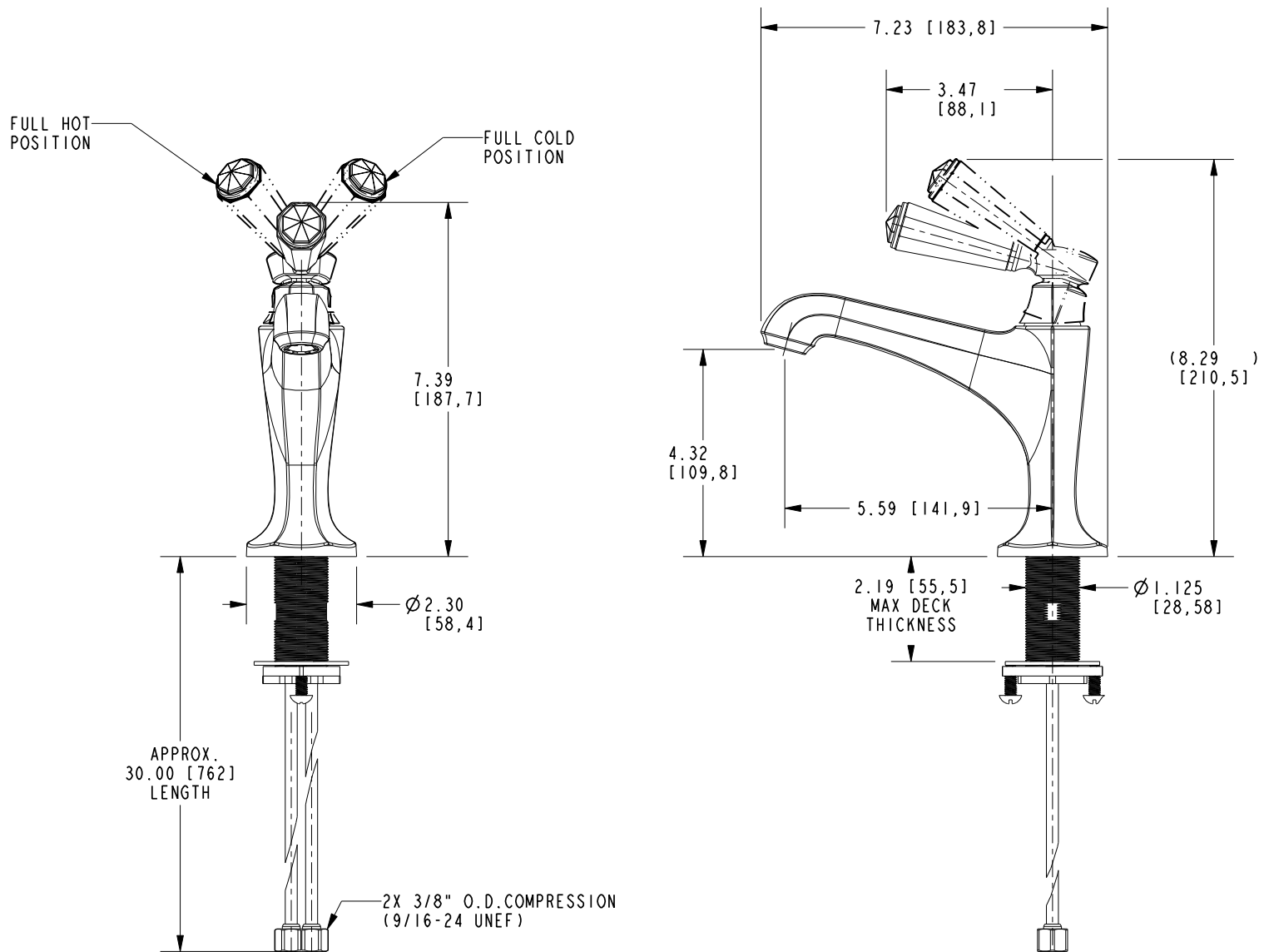
SINGLE HOLE LAVATORY FAUCET
