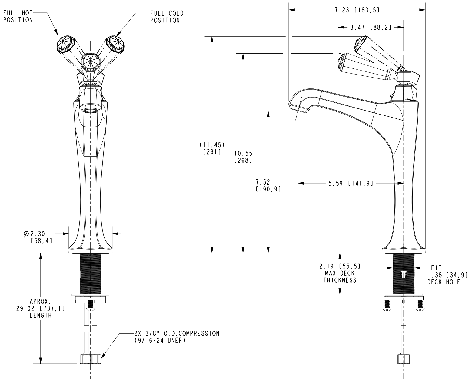
SINGLE HOLE VESSEL FAUCET
