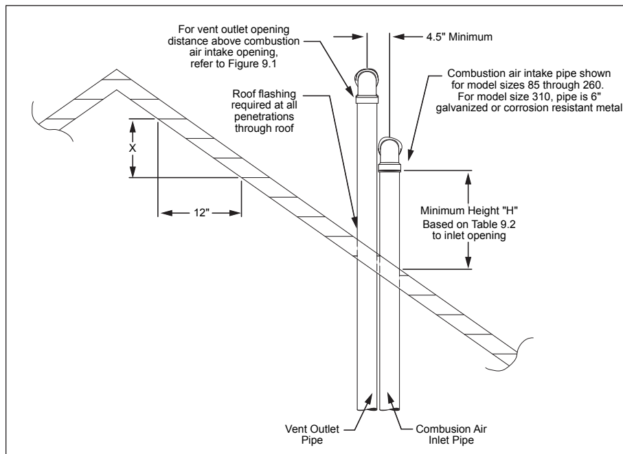
Figure 9.2 - Vertical 2-Pipe Vent System for Sloped Roofs
