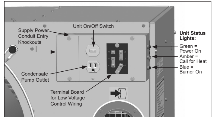
Figure 17.1 - Power/Control Wiring
