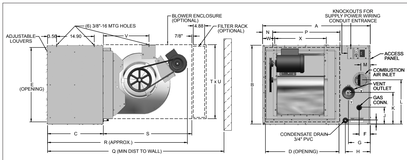
Figure 27.1 - Dimensional Drawings - Model BTC
