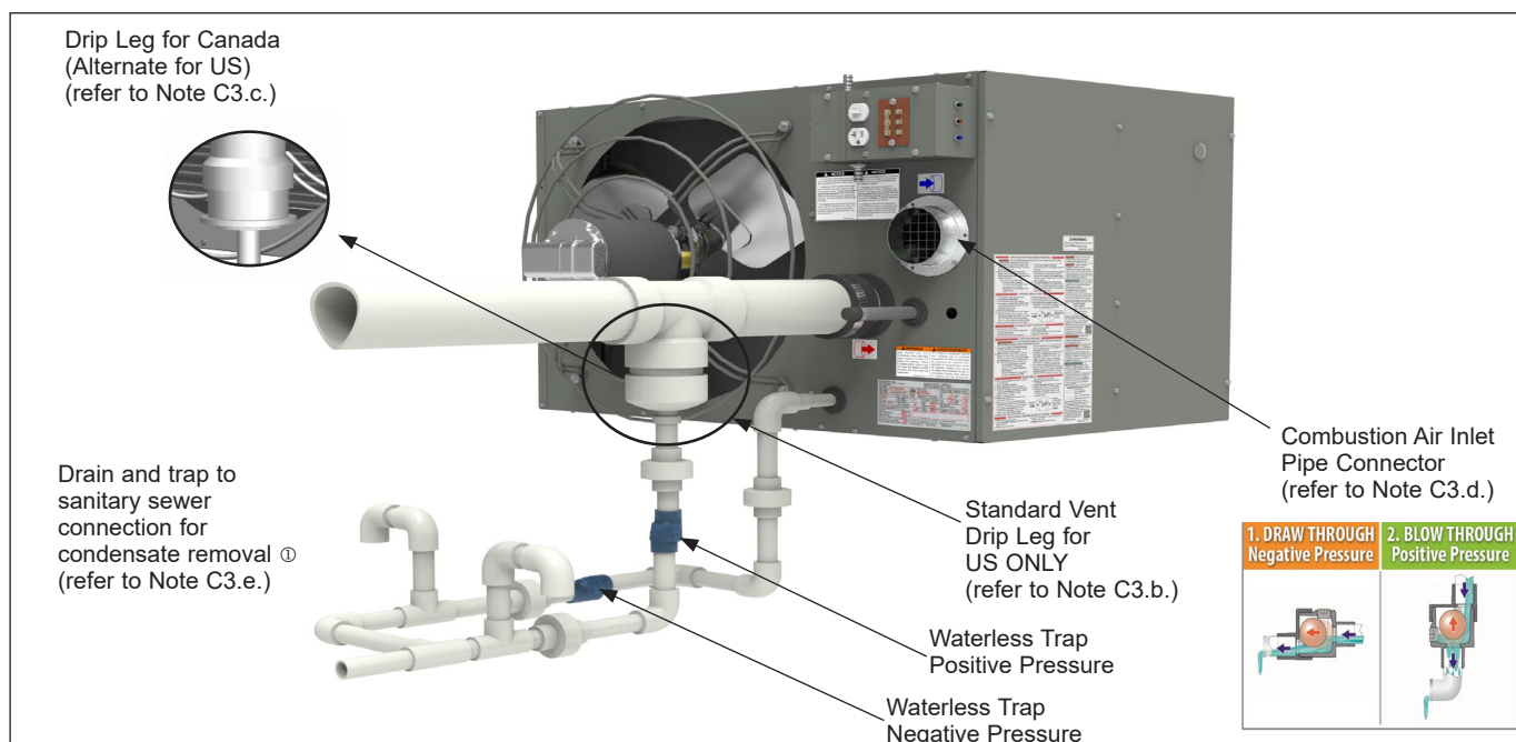
Figure 10.1 - Venting System Drip Leg and Condensate Drain Connections
