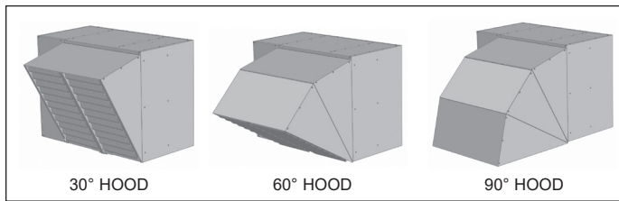
Figure 25.1 - 30°, 60°, & 90° Deflector Hoods
