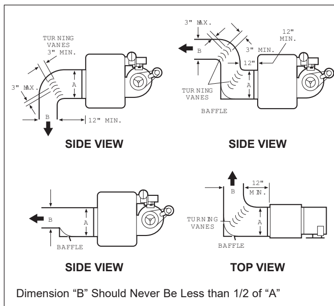
Figure 13.1 - Recommended Ductwork Installations
