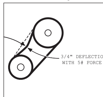
Figure 14.3 - Belt Tension Adjustment
