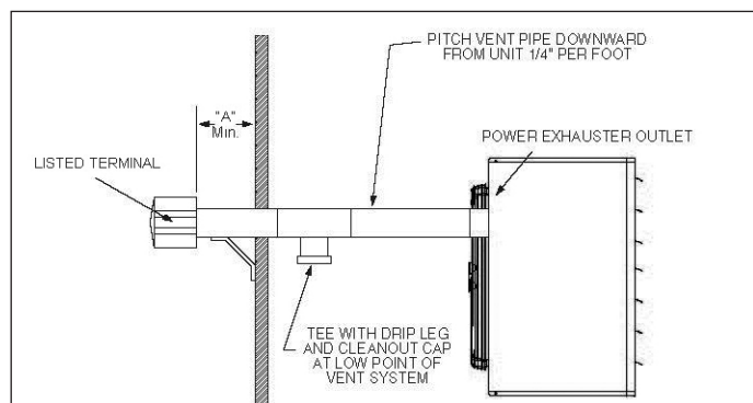
Figure 9.2 - Horizontal Venting
