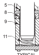
TYPICAL 14"-20" VALVE GROUNDING CONNECTION
