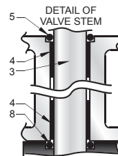
DETAIL OF VALVE STEM
