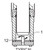
TYPICAL 24" VALVE GROUNDING CONNECTION
