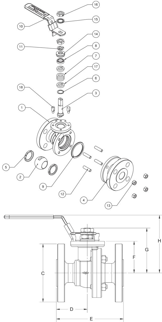
Class 150 # Dimensions
