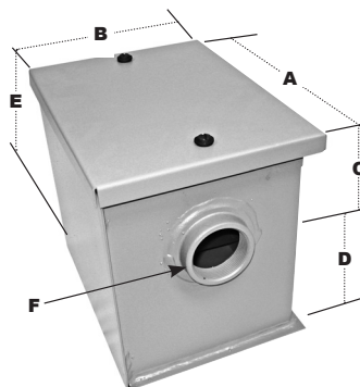
MI-GO-1 steel interceptor illustrated
