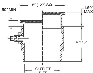
C224-30-S-1
