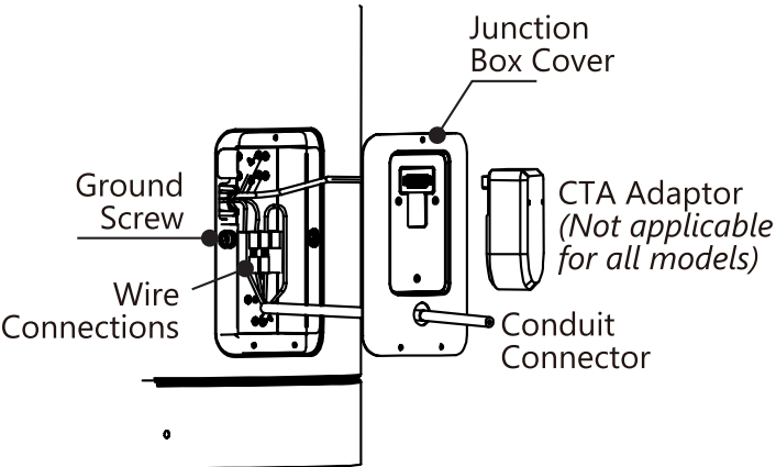
Junction Box Details
