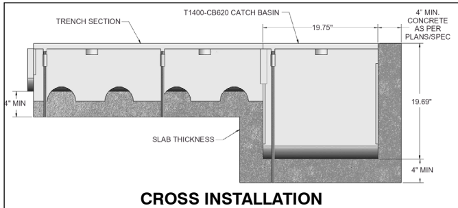
CROSS INSTALLATION
