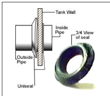
4" SLIP FIT CONNECTION
