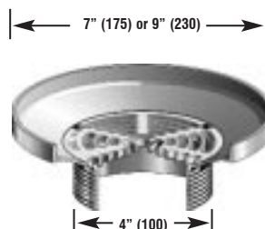
ER Indirect Waste Extended Rim Strainer
