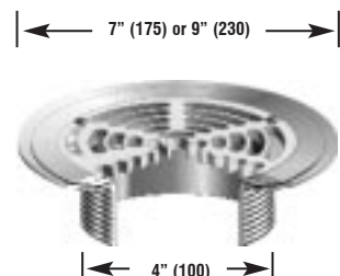
FC With Surface Membrane Clamp
