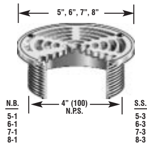
EG Indirect Waste Multi-Pipe Funnel
