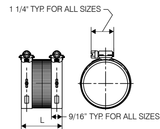
Sizes 2" through 4" Tighten bands alternately to recommended torque.
