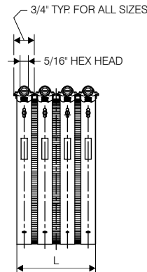
Sizes 5" through 10" Tighten inside bands first, then outside bands.
