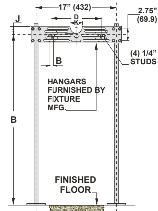
BASE DETAIL
