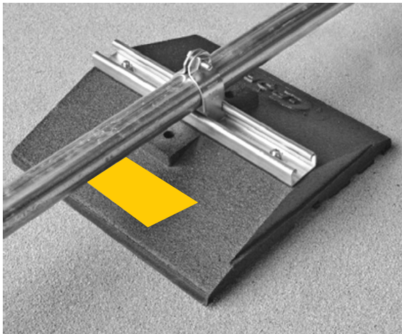
CW12 illustrated. Pipe clamp by others.
