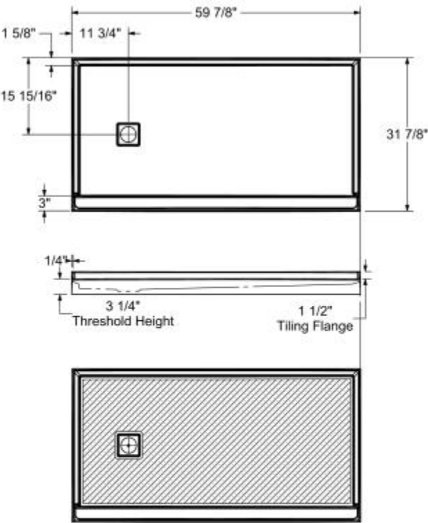
The hatched area represent the anti-slip surface
