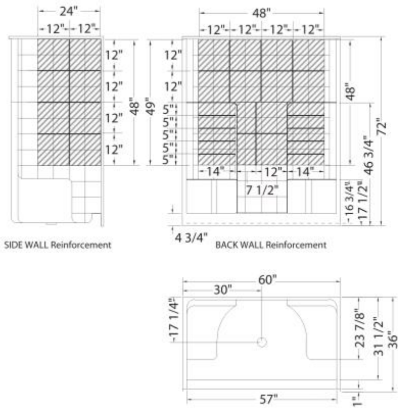
Full Wall Reinforcement Shown
