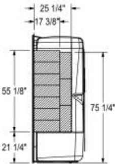
OPTIONAL REINFORCEMENT (Left shown, Right symmetrical)
