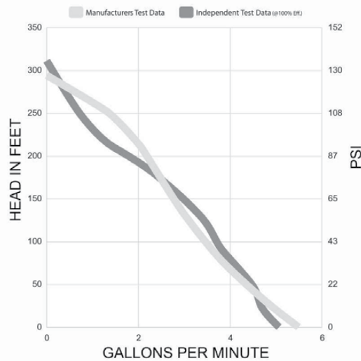
210w/36v 3" Solar Pump powered by 3x 12v Batteries (10ah)
