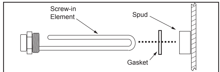
Figure 16. Heating Element Components
