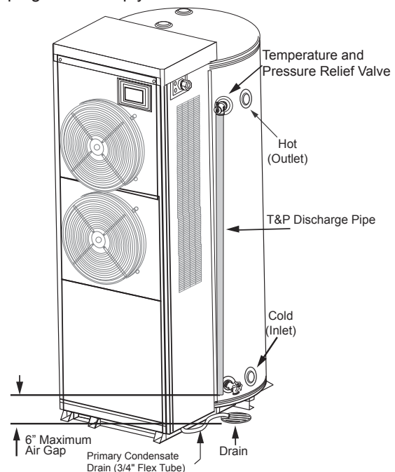
Figure 6. Condensate Tube Installation
