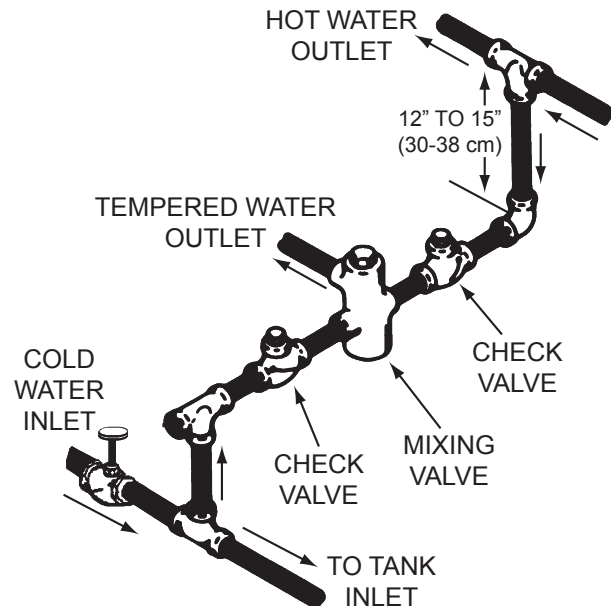
Figure 5. Mixing Valve
