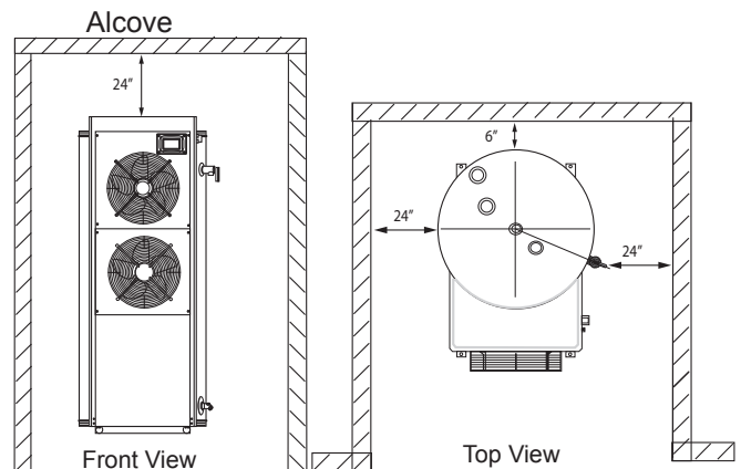
Figure 4. Clearances
