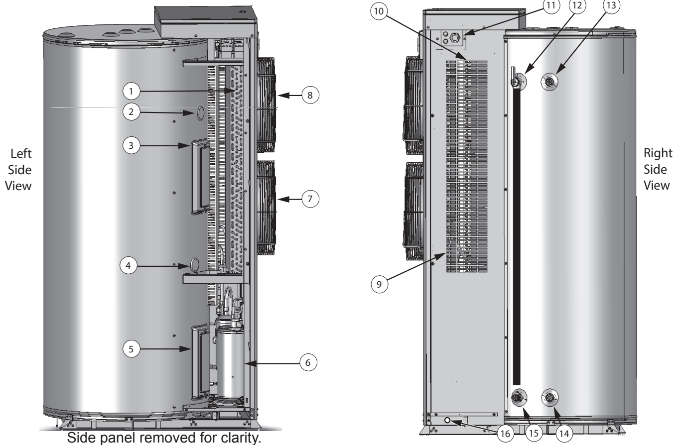
Figure 3. Left and Right Side Views
