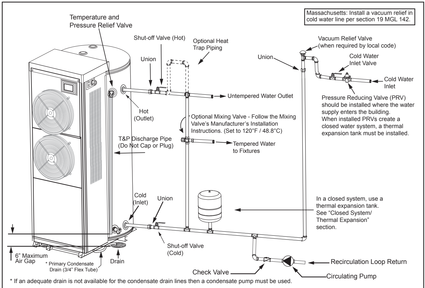
Figure 13. Completed Water System Piping
