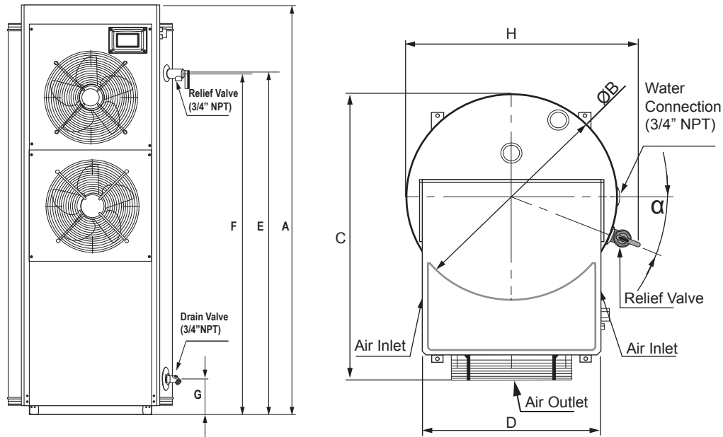
Figure 1. Rough-In Dimensions
