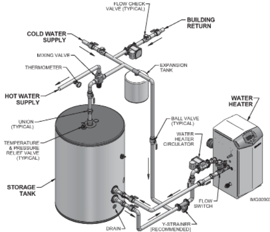
Figure 2-4_Vertical Tank Piping Diagram, Condensing
