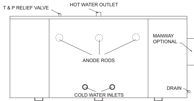
Figure 5-3_Horizontal Storage Tank w/Anodes
