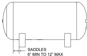
Figure 2-1_Saddle locations
