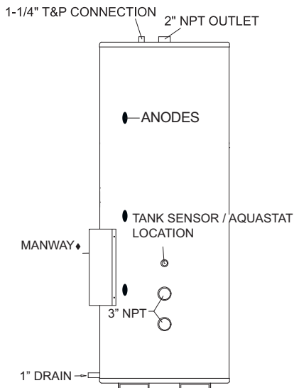
Figure 5-4_Vertical Storage Tank w/Anodes
