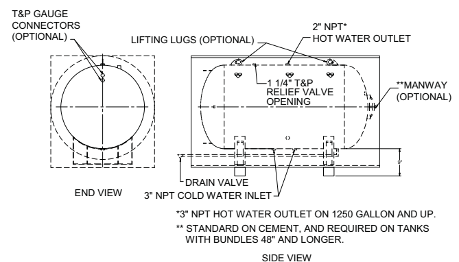
Figure 5-2_Horizontal Tank
