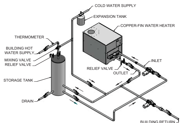
Figure 2-2_Vertical Tank Piping Diagram, Non-Condensing
