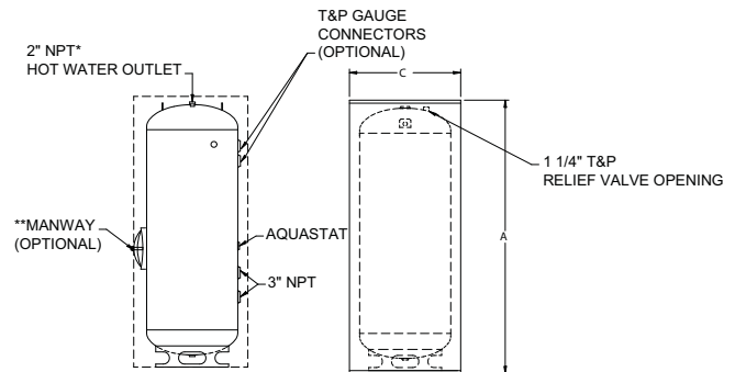
Figure 5-1_Vertical Tank
