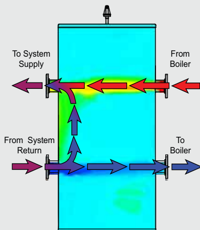
System Flow > Boiler Flow
