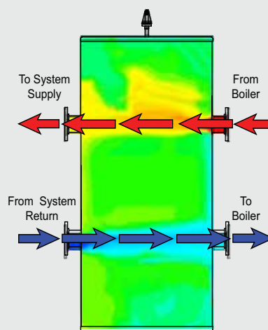
System Flow = Boiler Flow
