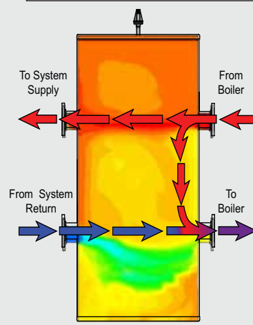
System Flow < Boiler Flow
