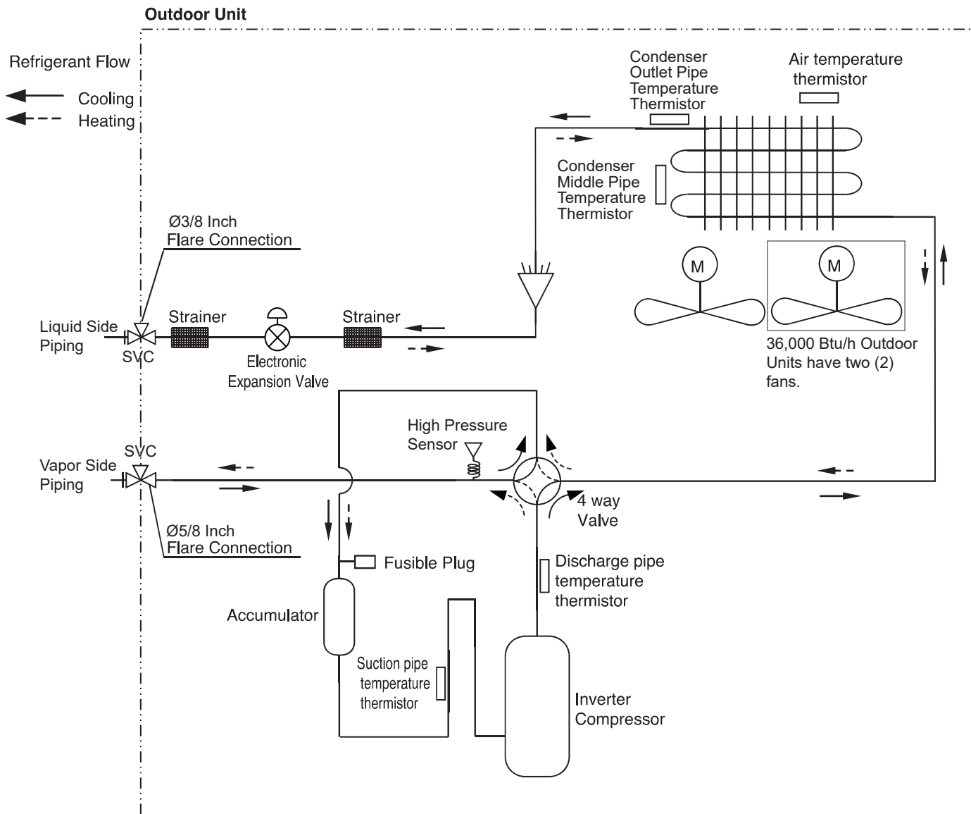
Figure 22: LUU180HHV, LUU240HHV, LUU360HHV Refrigerant Flow Diagram.
