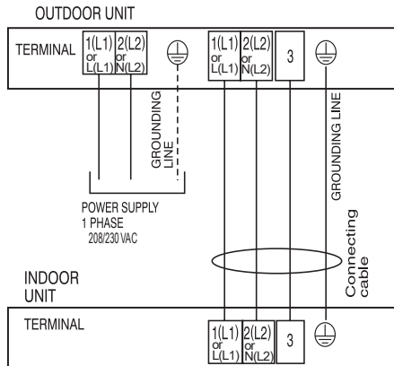
Figure 34: Schematic of a Single Zone Cassette System When the Wiring is GREATER THAN 130 Feet.
