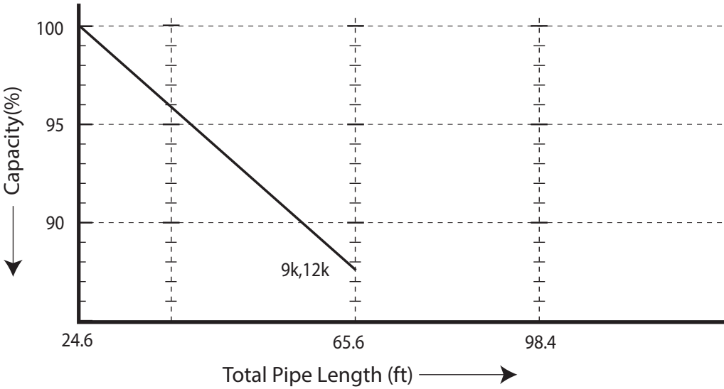
Figure 17: LS091HSV3, LS121HSV3 Cooling Coefficient Factor
