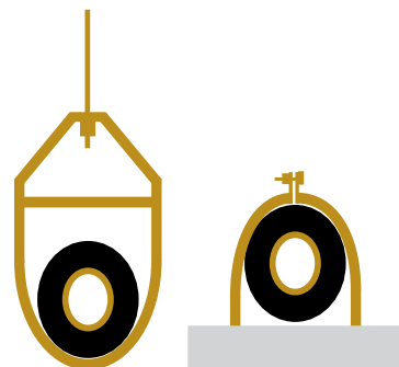
Figure 33: Typical Pipe Support Location—Change in Pipe Direction.
