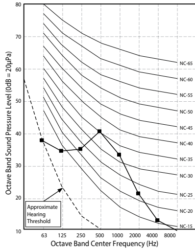
Figure 14: LSN240HLV
