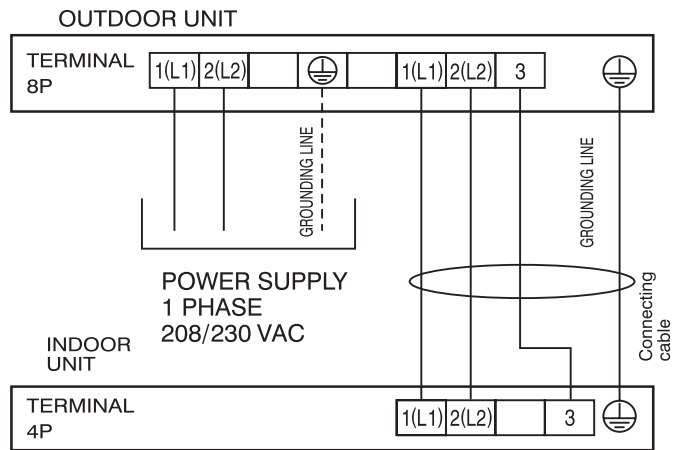
Figure 44: Terminal Block Wiring Diagram - LSU181HSV3, LSU240HSV3
