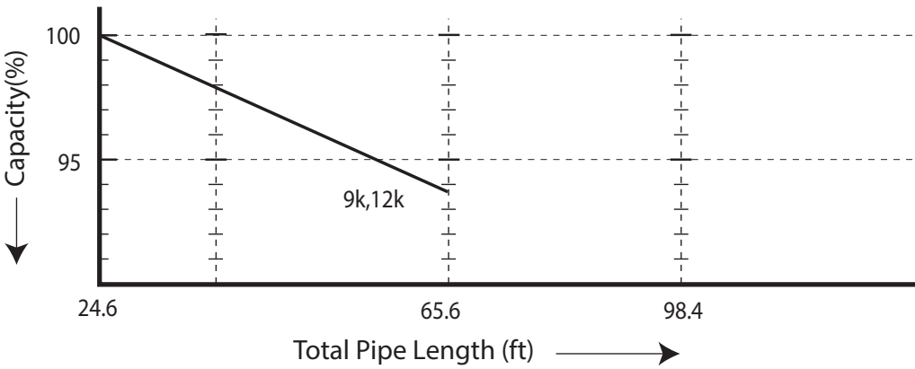
Figure 18: LS091HSV3, LS121HSV3 Heating Coefficient Factor
