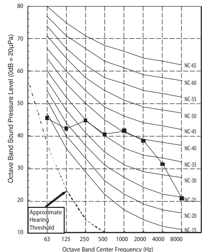
Figure 10: LSN181HSV3
