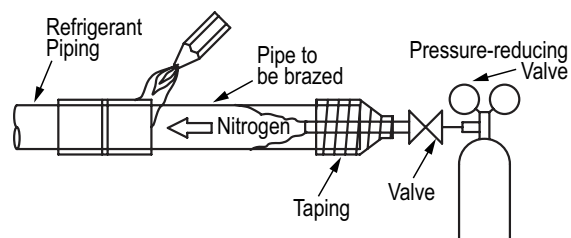
Figure 40: Refrigerant Pipe Brazing.
