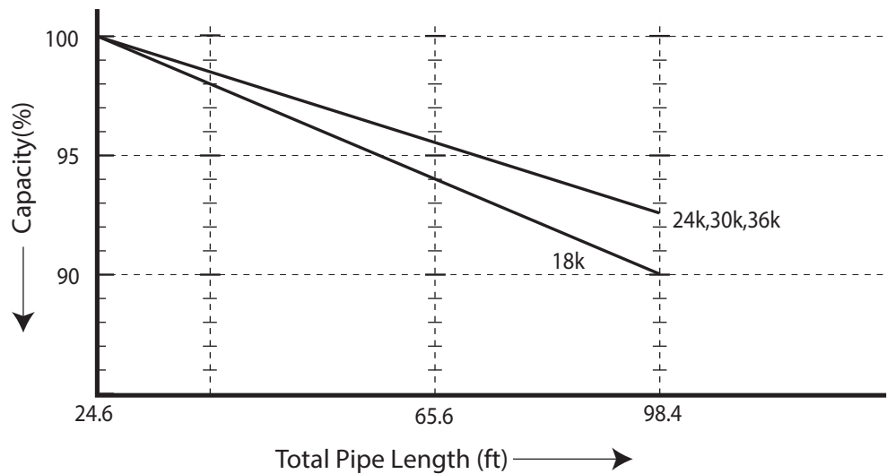
Figure 20: LS181HSV3, LS240HSV3, LS307HV3, LS360HV3 Heating Coefficient Factor
