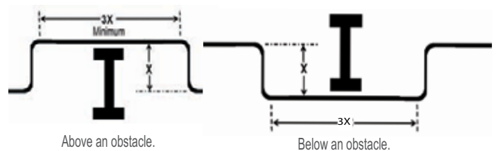
Figure 31: Installing Piping Above and Below an Obstacle
