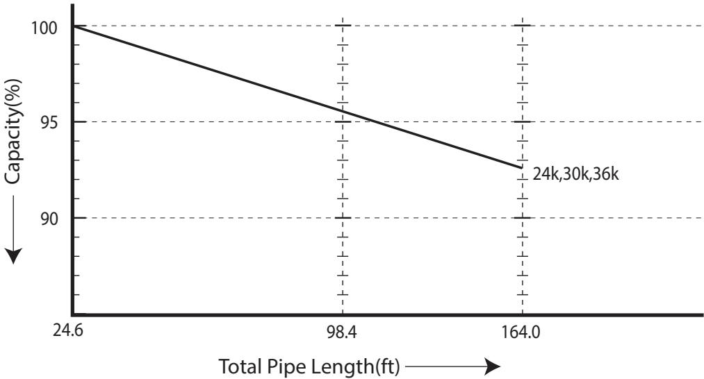
Figure 22: LS240HLV, LS300HLV, LS360HLV Heating Coefficient Factor
