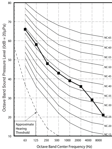
Figure 11: LSN240HSV3
