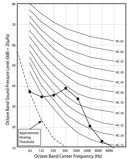
Figure 16: LSN360HLV
