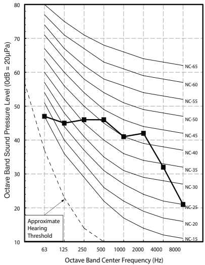
Figure 13: LSN360HSV3
