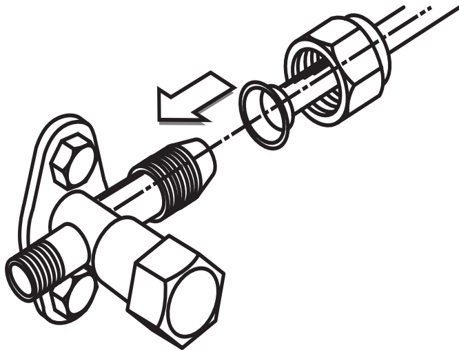
Figure 38: Pipe Attachment
