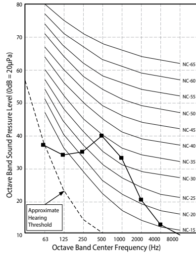
Figure 15: LSN300HLV
