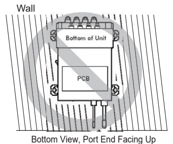
Figure 39: Unacceptable Branch Distribution Unit Orientation.
