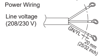
Figure 40: Multi F / Multi F MAX Outdoor Unit Power Wiring.
