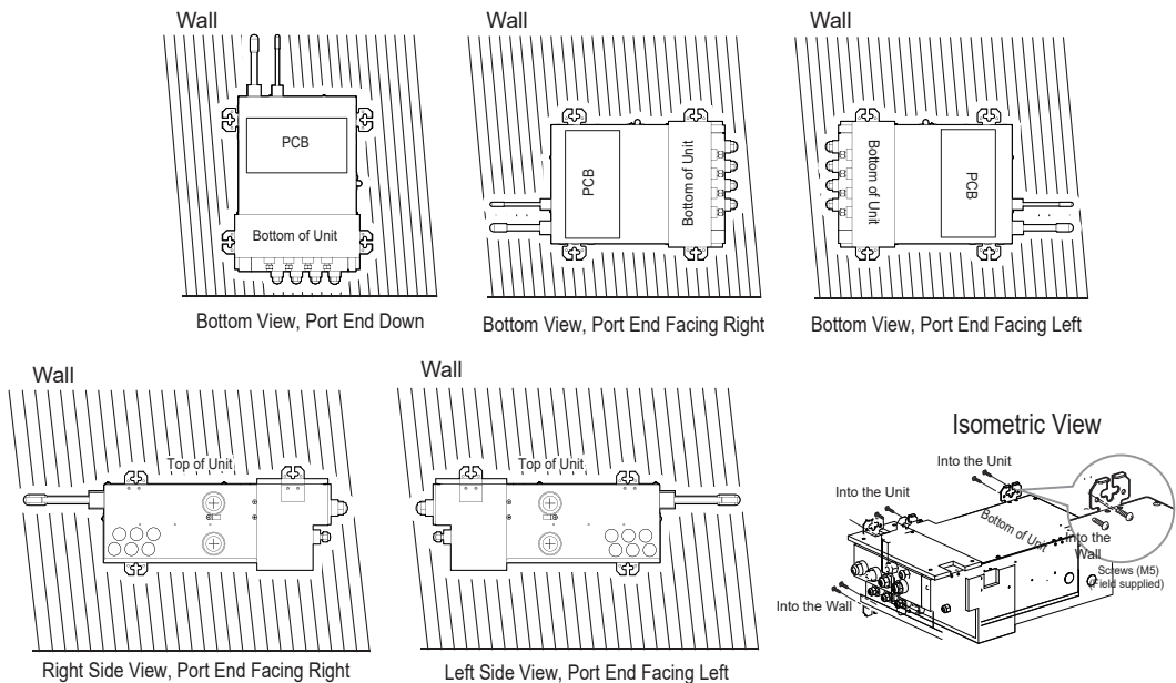
Figure 38: Acceptable Branch Distribution Unit Wall Mount Orientations.
