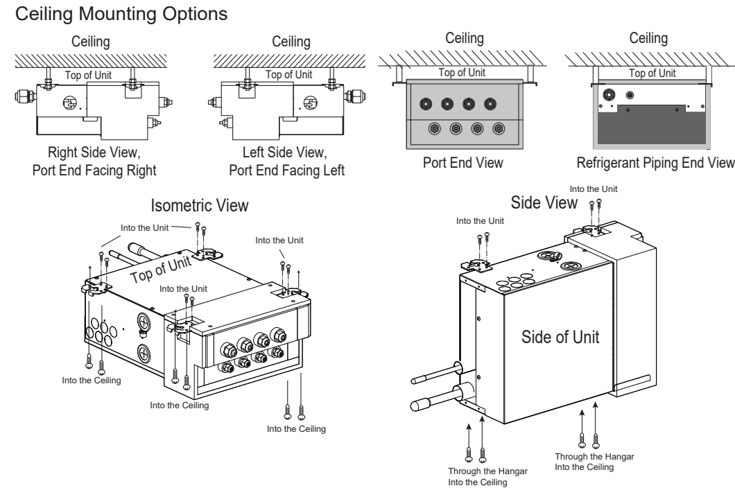
Figure 37: Acceptable Branch Distribution Unit Ceiling Mount Orientations.
