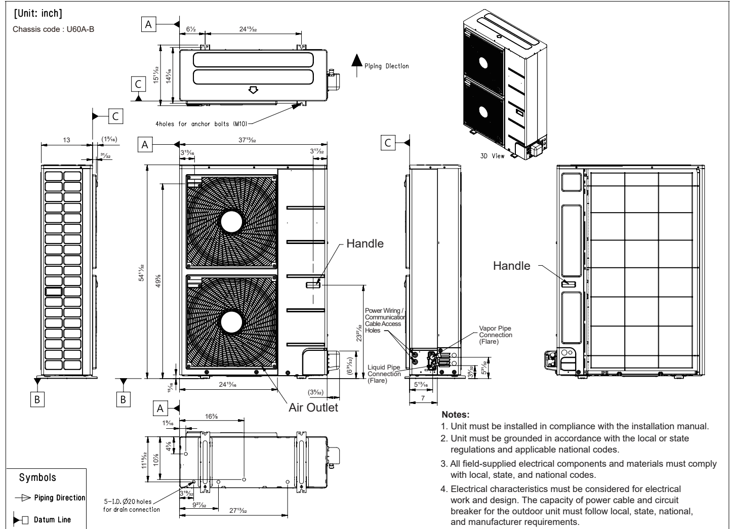
Figure 18: KUMXB601A Dimensions.
