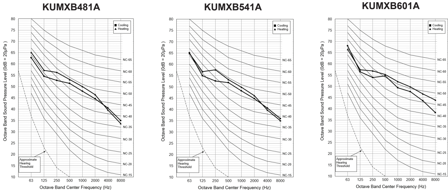
Figure 25: Sound Pressure Diagrams.
