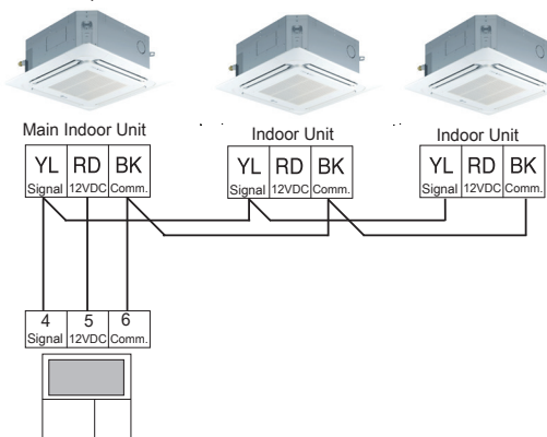
Figure 50: Example of Indoor Unit Group to Zone Controller Connections (Sig-12V-GND [Comm.] Terminal).
