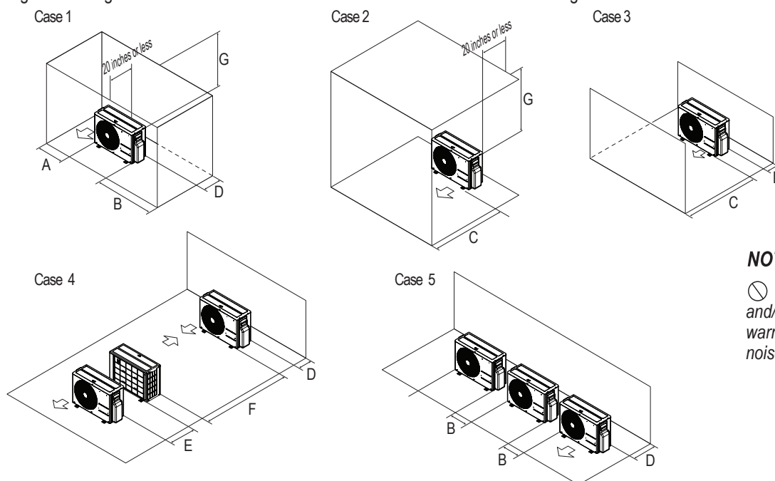
Figure 57: Single Fan Outdoor Unit Service Access and Allowable Clearances Diagram.
