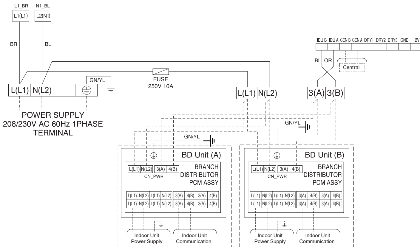
Figure 39: Multi F MAX with LGRED KUMXA181A, KUMXA241A, and KUMXA301A System Power Wiring and Communications Cable.
