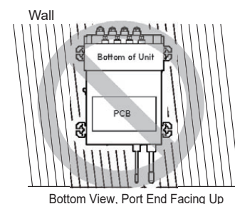
Bottom View, Port End Facing Up
