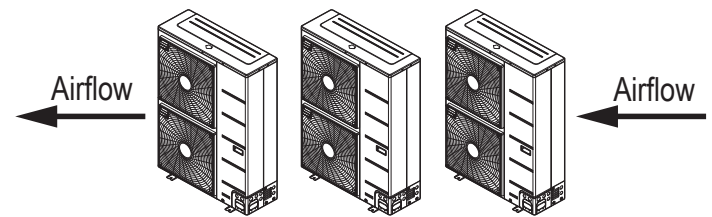
Figure 51: Proper Outdoor Unit Placement and Clearances When There Are Obstacles on the Suction Side.
