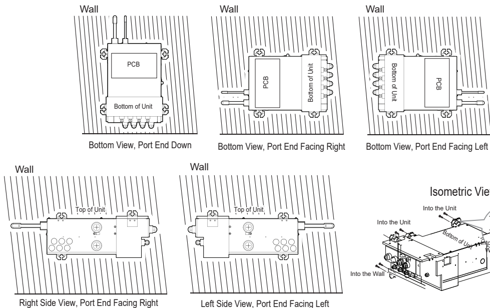
Figure 31: Acceptable Branch Distribution Unit Wall Mount Orientations.
