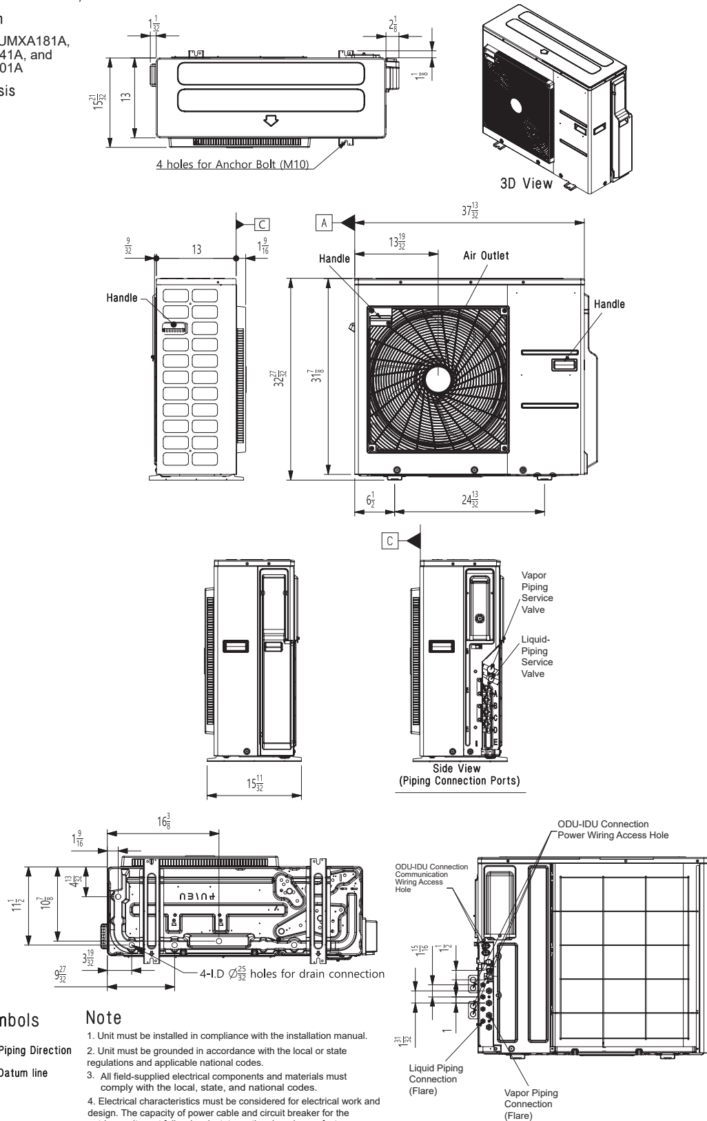
Figure 4: KUMXA181A, KUMXA241A, KUMXA301A Dimensions.
