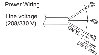
Figure 33: Multi F / Multi F MAX with LGRED Outdoor Unit Power Wiring.
