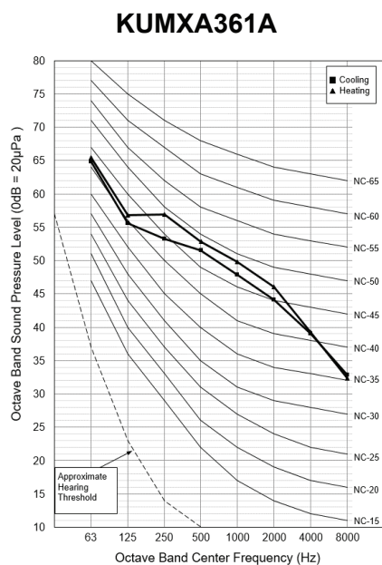
Figure 19: Sound Pressure Level Diagrams.
