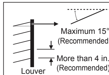
Figure 54: Louver Recommendations.
