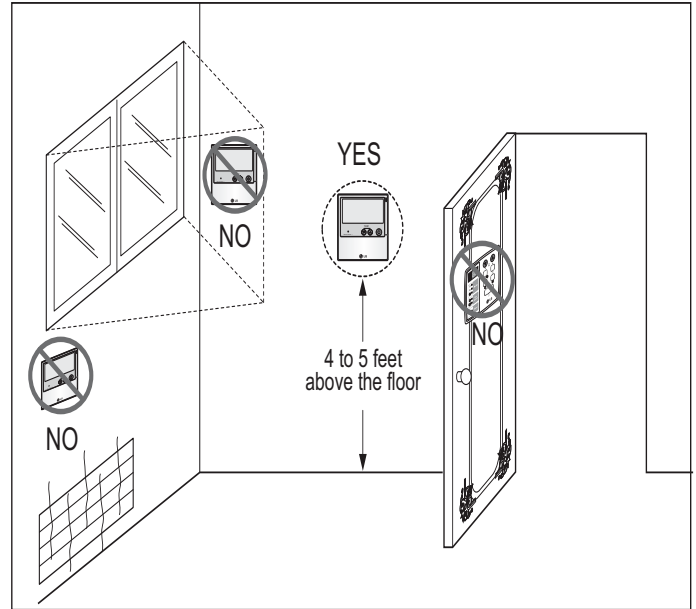
Figure 67: Proper Location for the Wired Controller.
