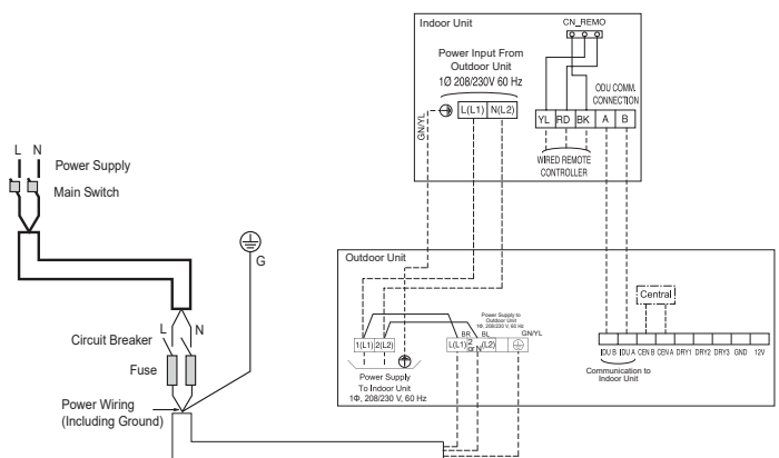
Figure 60: General R32 Single-Zone System Power / Communications System Schematic (Appearances May Vary).
