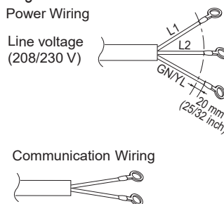
Figure 61: R32 Single Zone Outdoor Unit to Indoor Unit Wiring and Communications Cable Diagram.
