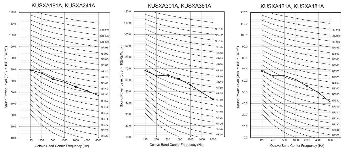
Figure 18: LGRED Four-Way Ceiling Cassette Outdoor Unit Sound Power Level Diagrams.
