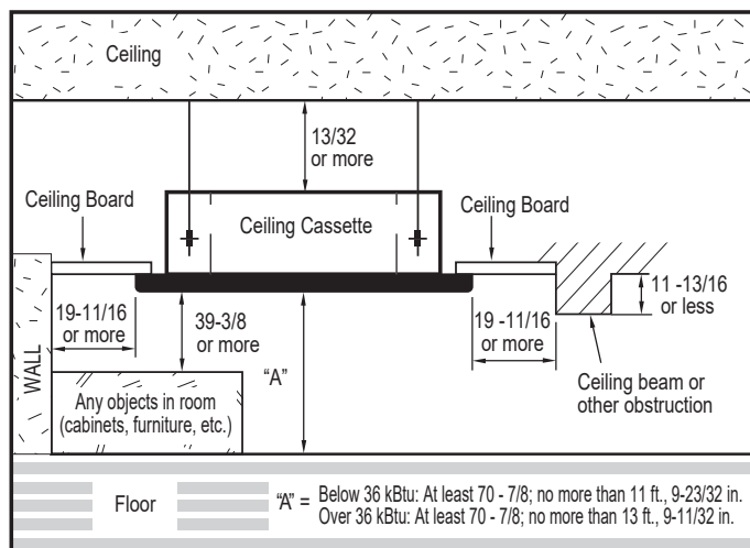
Figure 22: Cassette Indoor Unit Clearance Requirements.
