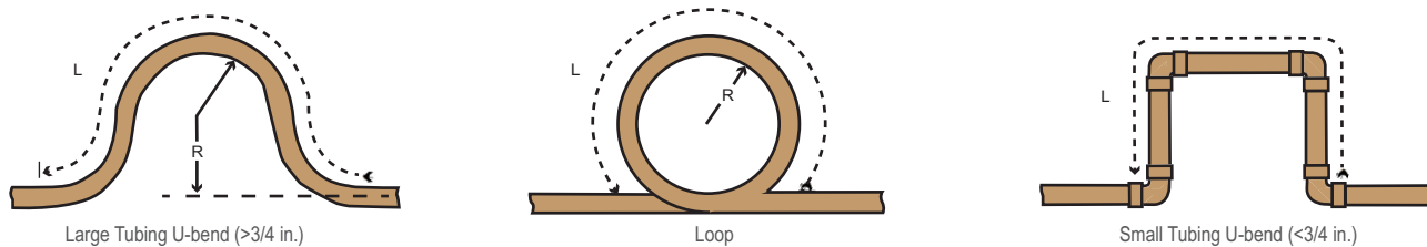
Figure 46: Coiled Expansion Loops and Offsets (Plan View).
