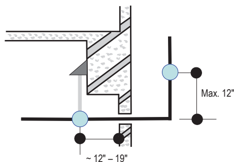
Figure 49: Typical Pipe Support Location—Change in Pipe Direction.
