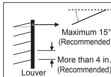
Figure 36: Louver Recommendations.
