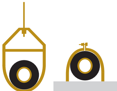
Figure 48: Pipe Hanger Details.
