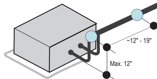
Figure 50: Pipe Support at Indoor Unit.
