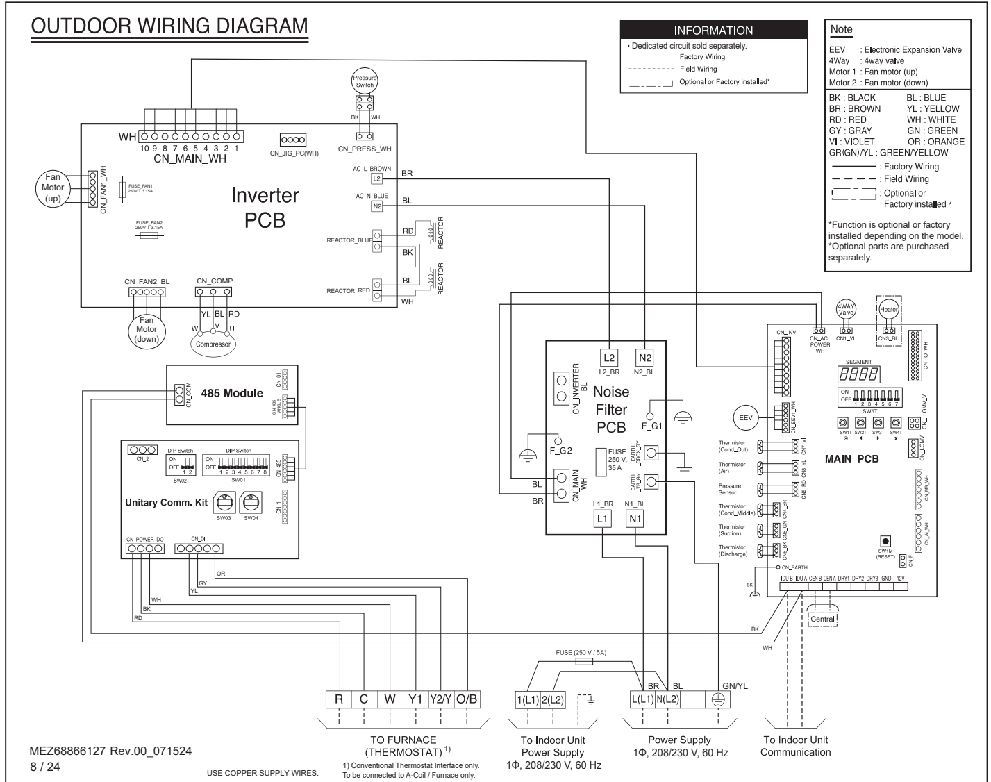
Figure 53: KUSXA301A, KUSXA361A Outdoor Unit Wiring Diagram.
