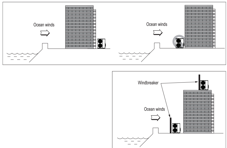
Figure 30: Oceanside Placement Using a Building as Shield, and Placement Using a Windbreak.
