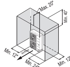
Single Unit—High Rear and Side Walls with Building Overhang
