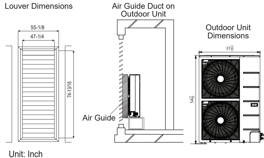
Figure 38: Example of Installing Outdoor Unit Indoors.
