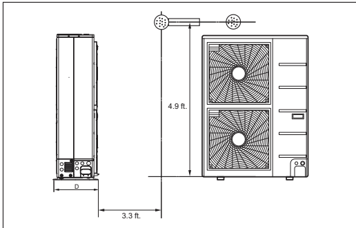
Figure 16: LGRED Four-Way Cassette Outdoor Unit Sound Pressure Level Measurement Location (For Illustrative Purposes Only; Appearance Depends on Model).
