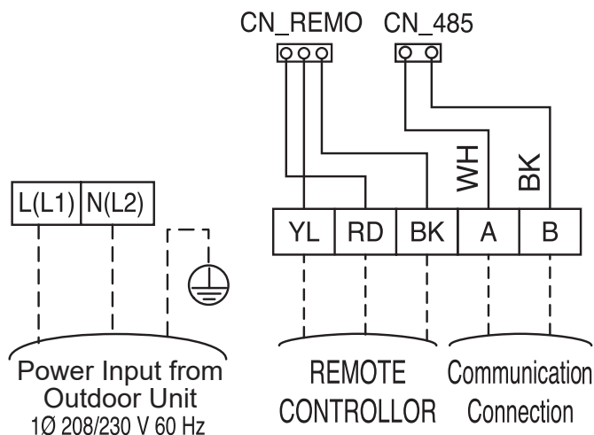
Figure 65: Wired Controller Connection (Example Only).
