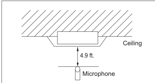
Figure 19: LGRED Four-Way Cassette Indoor Unit Sound Pressure Level Measurement Location.
