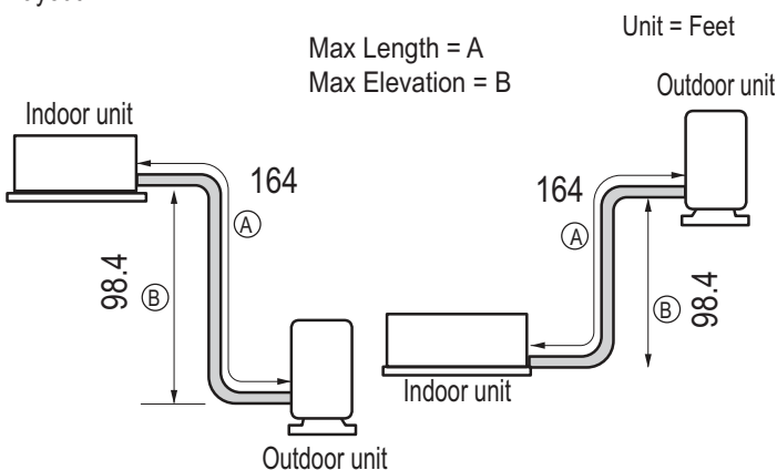
Figure 44: Typical KSUDA181A, KSSCA241A, KSSCA301A System Layout.
