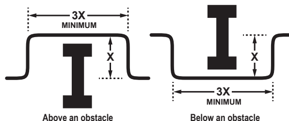
Figure 47: Installing Piping Above and Below an Obstacle.
