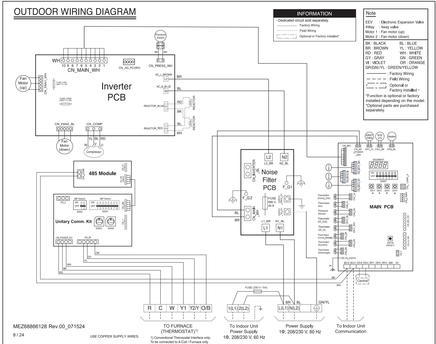
Figure 54: KUSXA421A, KUSXA481A Outdoor Unit Wiring Diagram.
