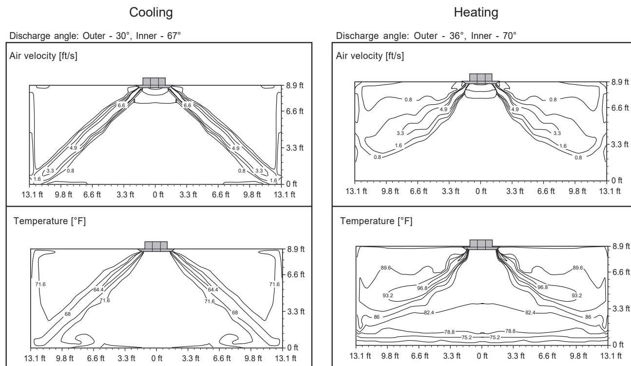
Figure 13: KNSCB241A Air Velocity and Temperature Distribution Charts.
