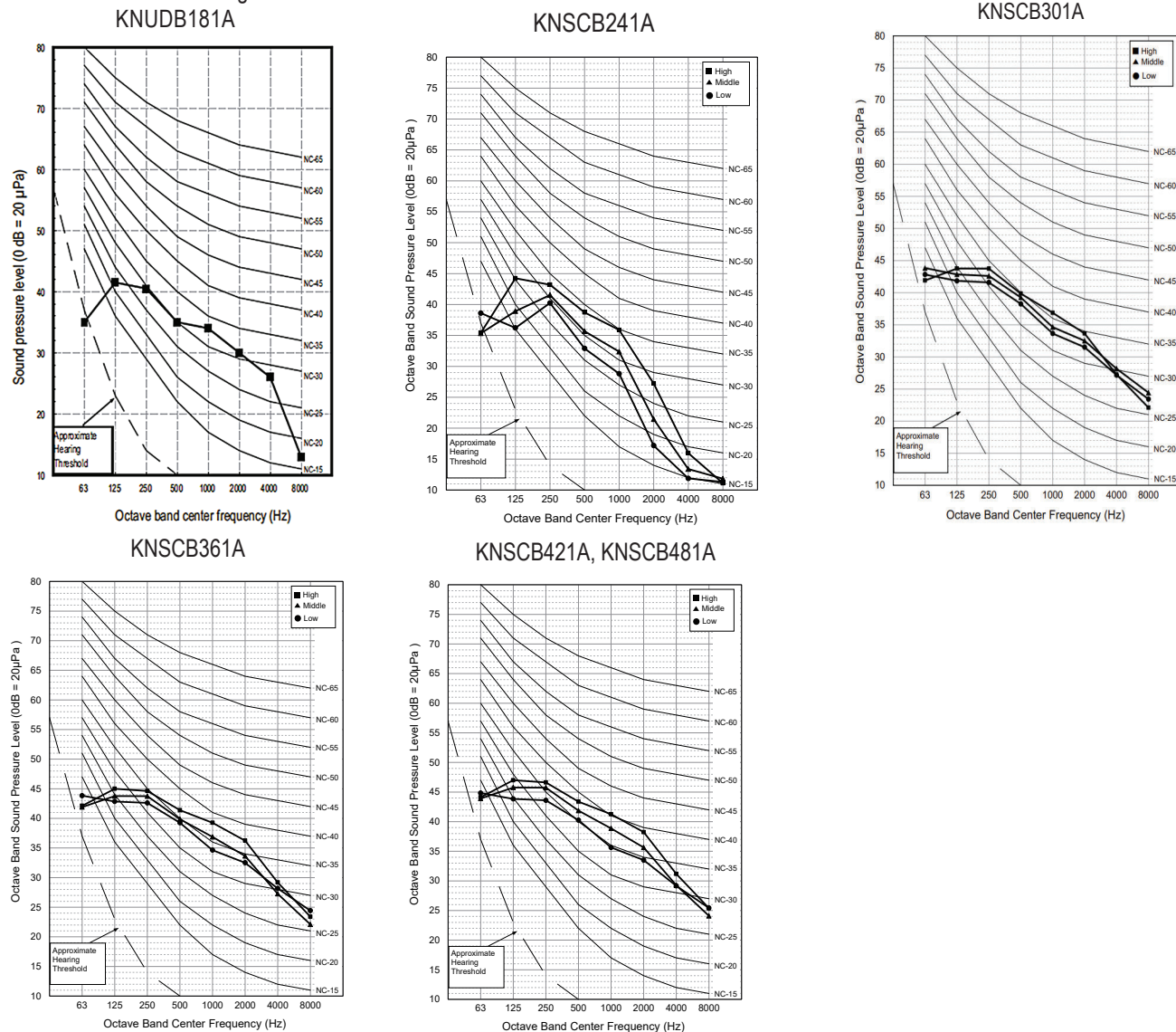
Figure 20: LGRED Four-Way Cassette Indoor Unit Sound Pressure Level Diagrams.
