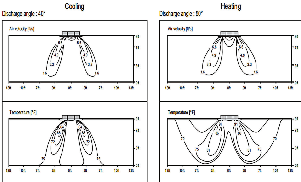
Figure 12: KNUDB181A Air Velocity and Temperature Distribution Charts.
