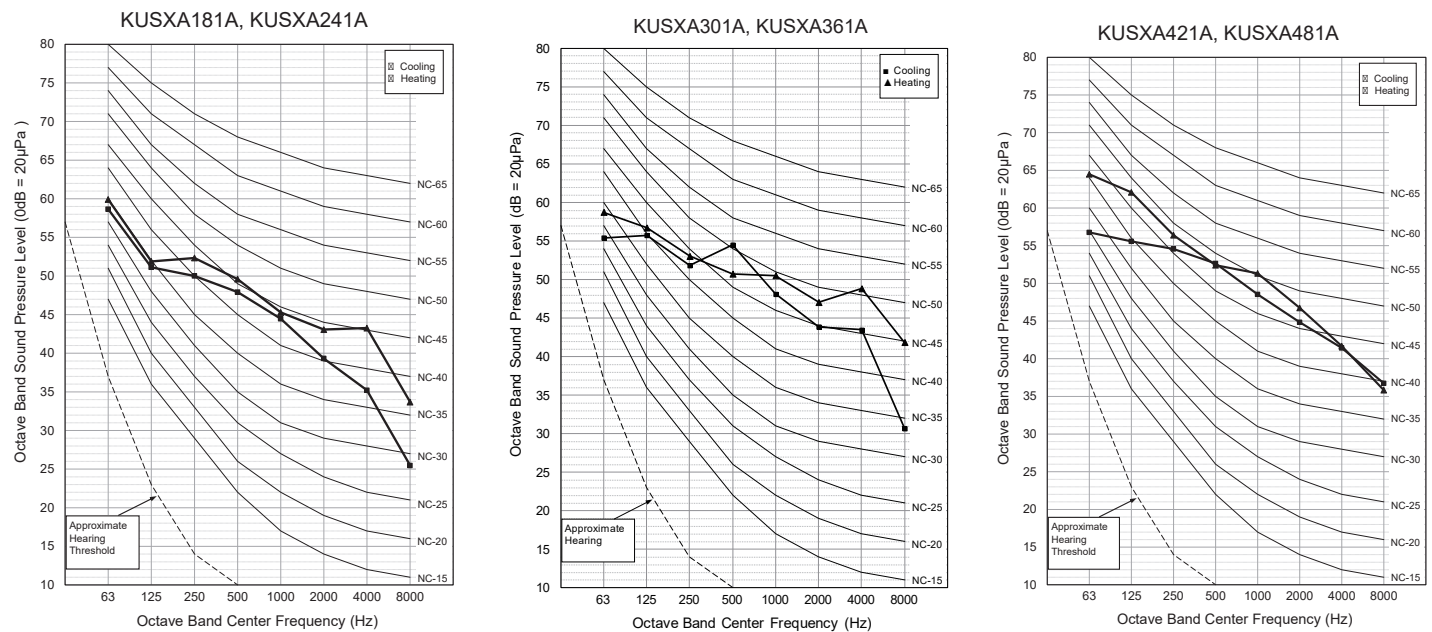
Figure 17: LGRED Four-Way Cassette Outdoor Unit Sound Pressure Level Diagrams.
