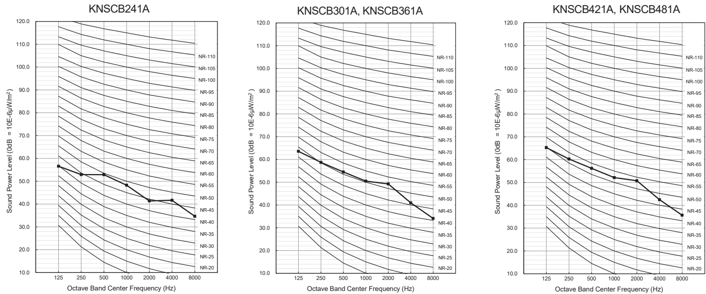
Figure 21: LGRED Four-Way Cassette Indoor Unit Sound Power Level Diagrams.
