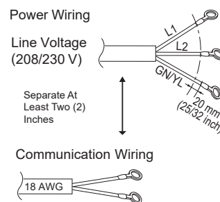
Figure 63: R32 Single-Zone Outdoor Unit to Indoor Unit Wiring and Communications Wiring Diagrams GREATER THAN 130 feet.
