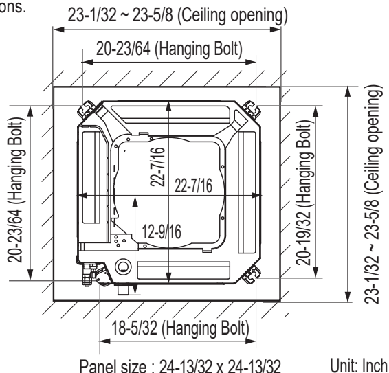
Figure 23: 2 x 2 Cassette Ceiling Opening Dimensions and Bolt Locations.
