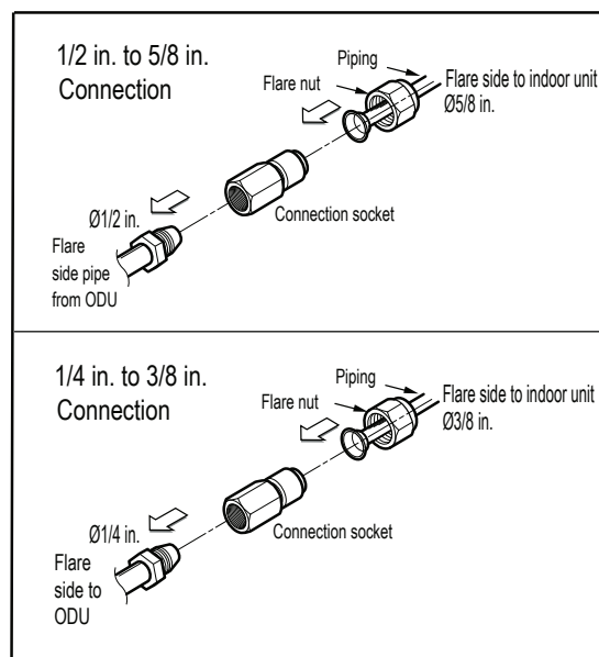
Figure 41: KNUDB181A Refrigerant Pipe Connections.
