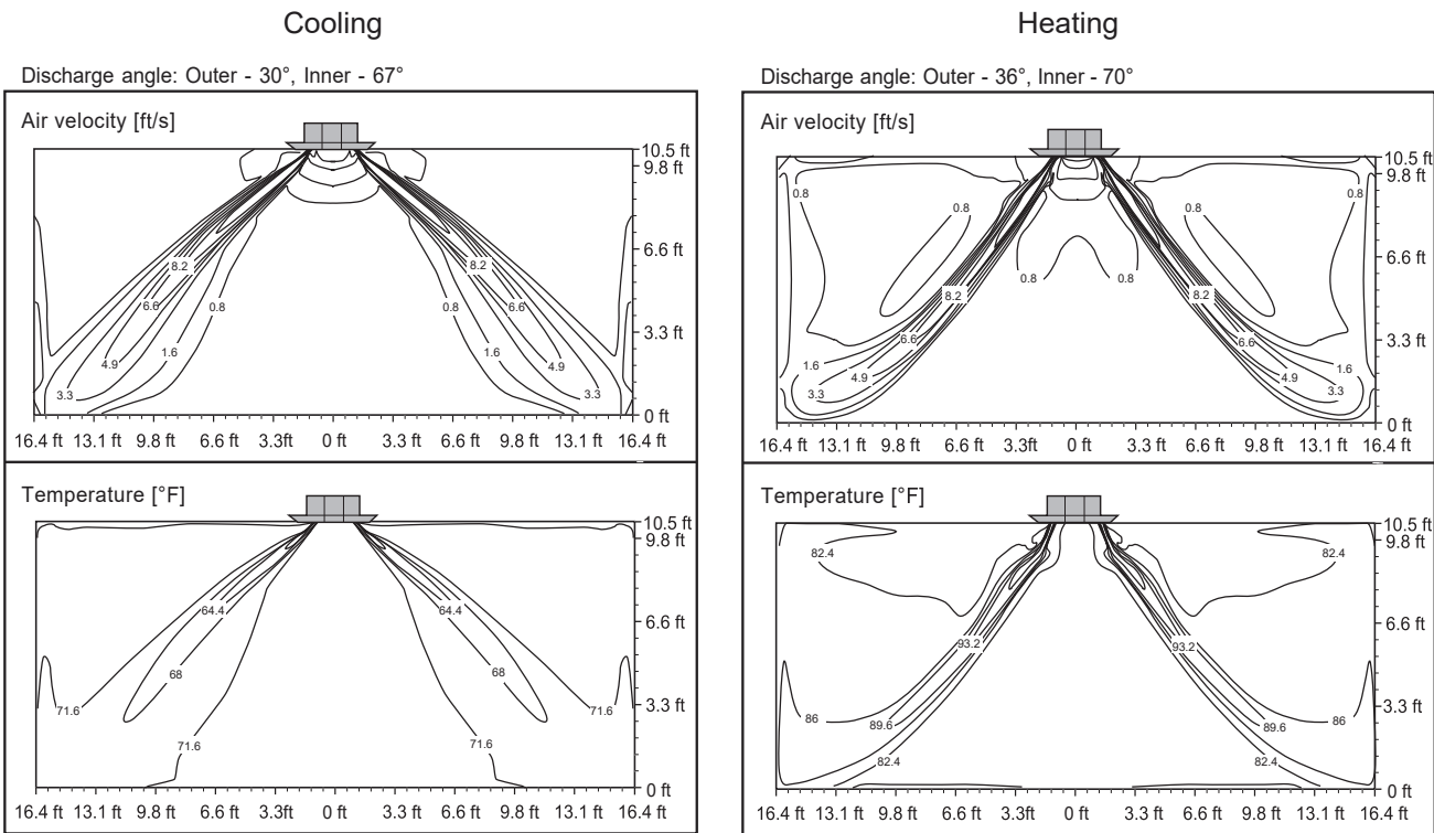
Figure 15: KNSCB421A, KNSCB481A Air Velocity and Temperature Distribution Charts.
