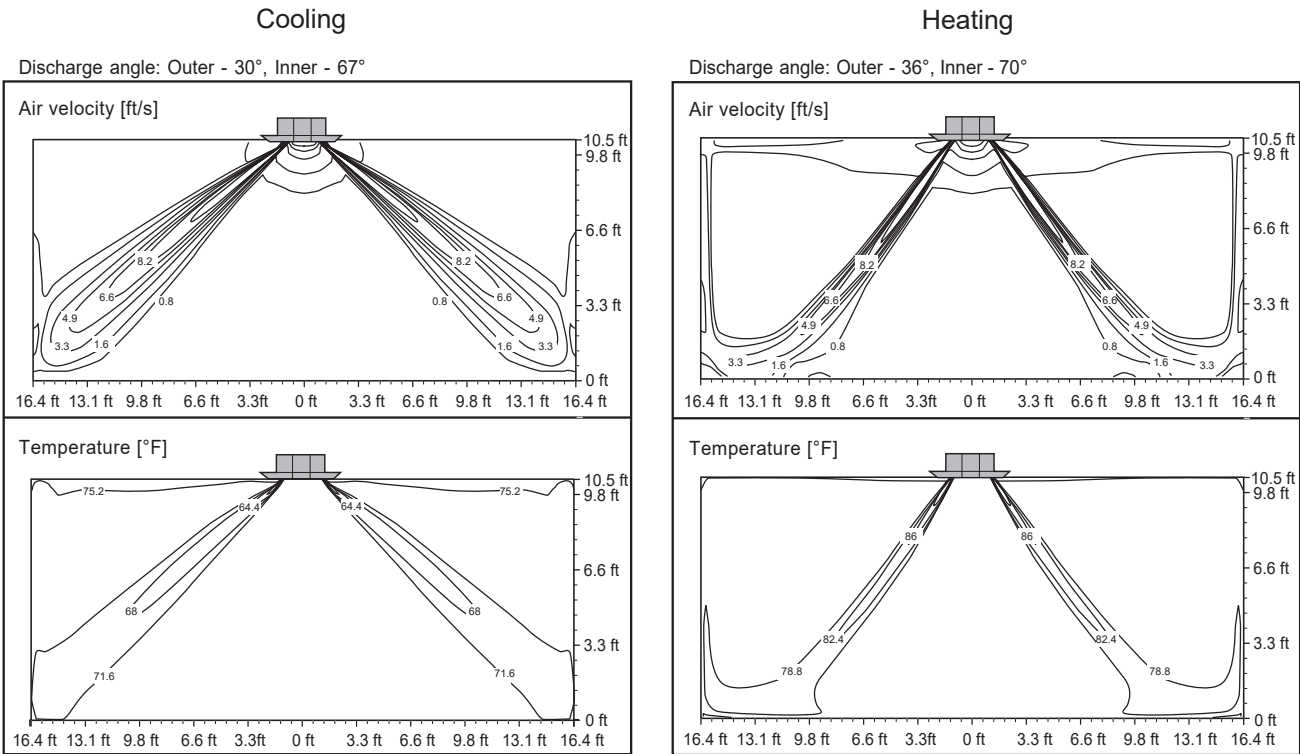
Figure 14: KNSCB301A, KNSCB361A Air Velocity and Temperature Distribution Charts.
