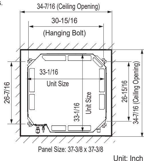
Figure 24: 3 x 3 Cassette Ceiling Opening Dimensions and Bolt Locations.
