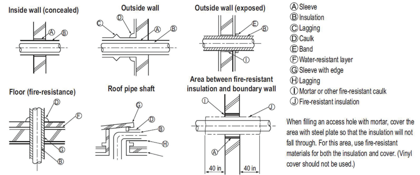
Figure 51: Pipe Sleeve Options.
