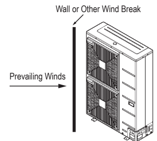
Figure 30: Oceanside Placement Using a Building as Shield, and Placement Using a Windbreak.
