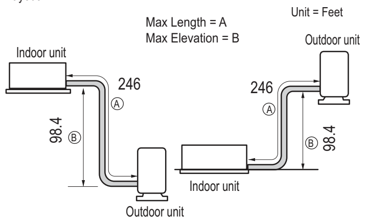
Figure 45: Typical KSSCA361A, KSSCA421A, KSSCA481A System Layout.
