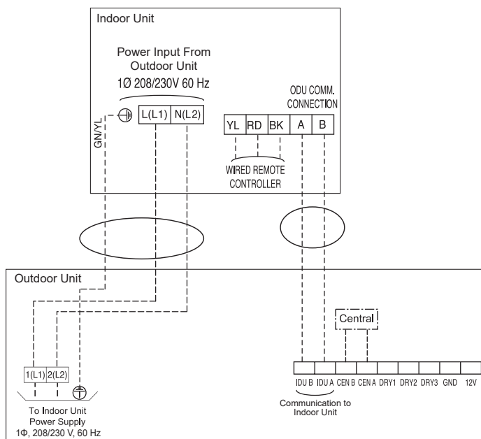
Figure 62: R32 Single Zone Power / Communication System Diagram (Appearances May Vary Slightly).
