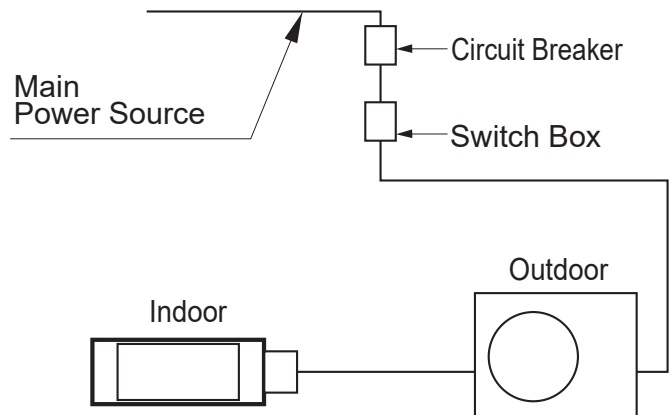
Figure 58: Circuit Breaker.
