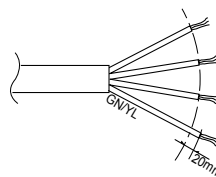
NORMAL CROSS-SECTIONAL AREA 0.75mm 2
