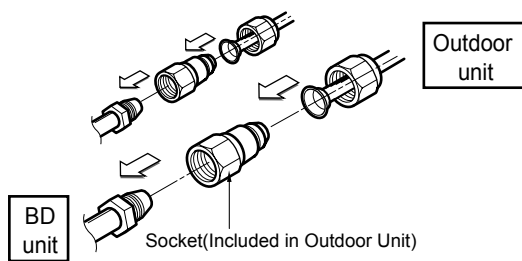
[Connector]
