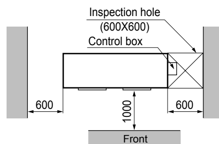
Top view (unit: mm)
