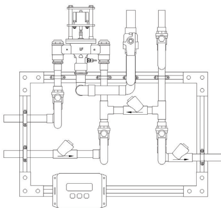
PNV-100-LF-R34 Enhanced Recirculation
