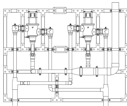
PNV-150-LF-2PS High Capacity
