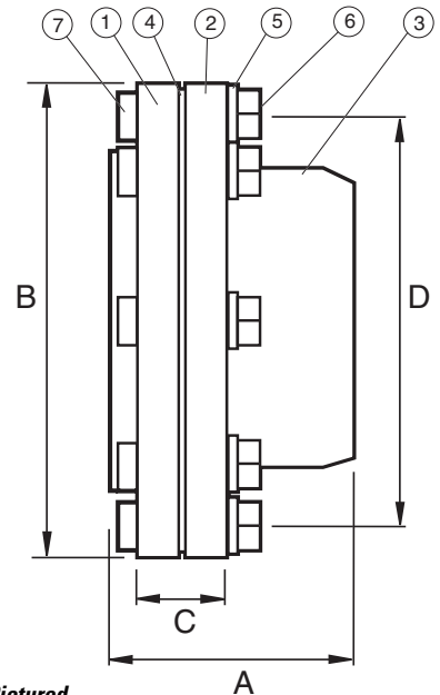
Pictured 4" T-571NL (Large Diameter) Cut-away
