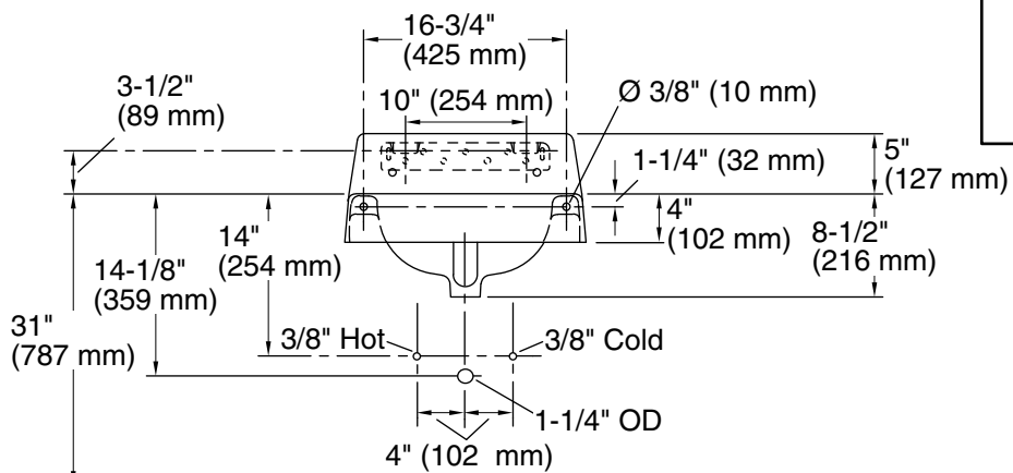
Standard Installation
