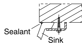
Sealant Sink Wood Counter Installation
