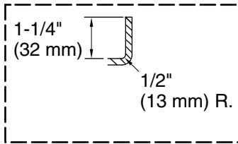
Integral Flange Detail
