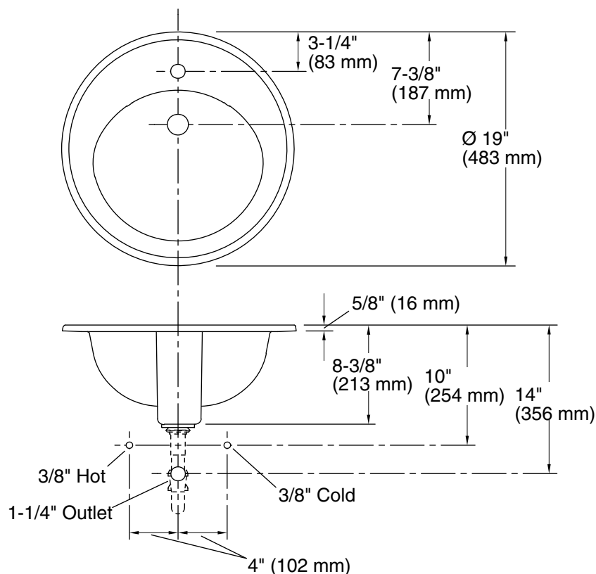
Standard Installation
