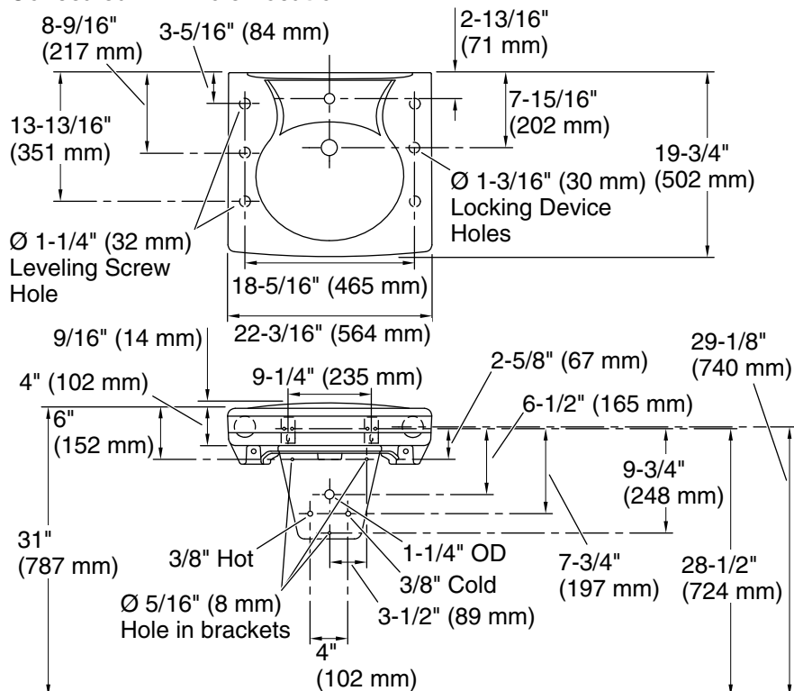
Recommended ADA/TAS Installation
