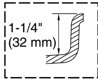
Rim Detail
