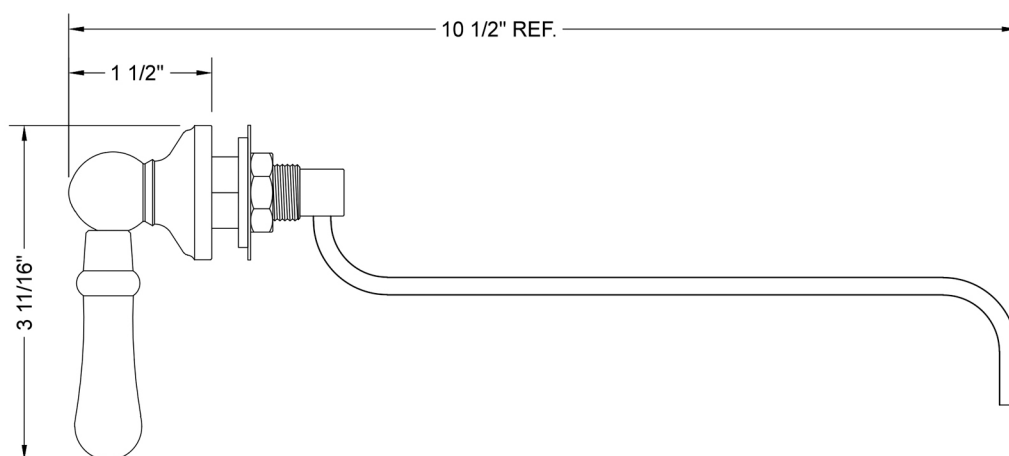
SIDE VIEW
