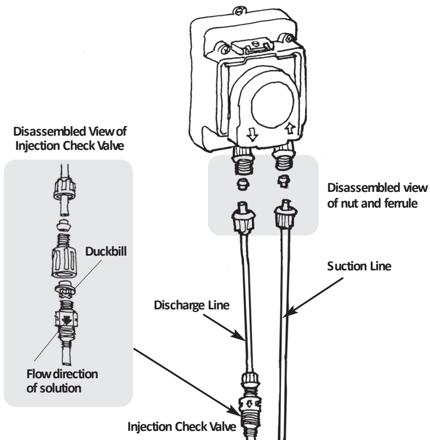
Figure 3: Chemical Pump Installation Diagram
