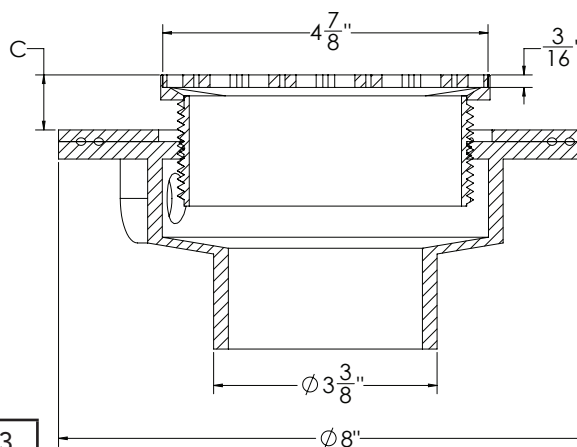
SECTION 1-1
