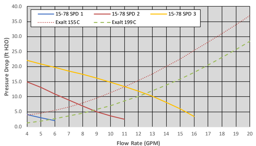
Exalt Combi Pump Curve
