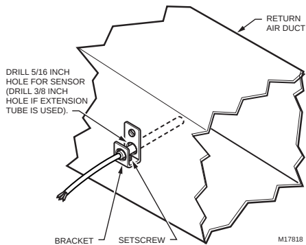
Fig. 2. Duct mounting with mounting bracket.
