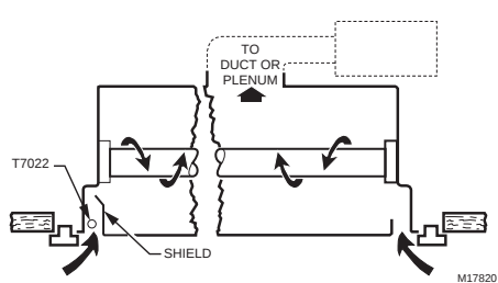
Fig. 5. Cross section of light troffer showing a typical mounting location at the end of the light troffer.
