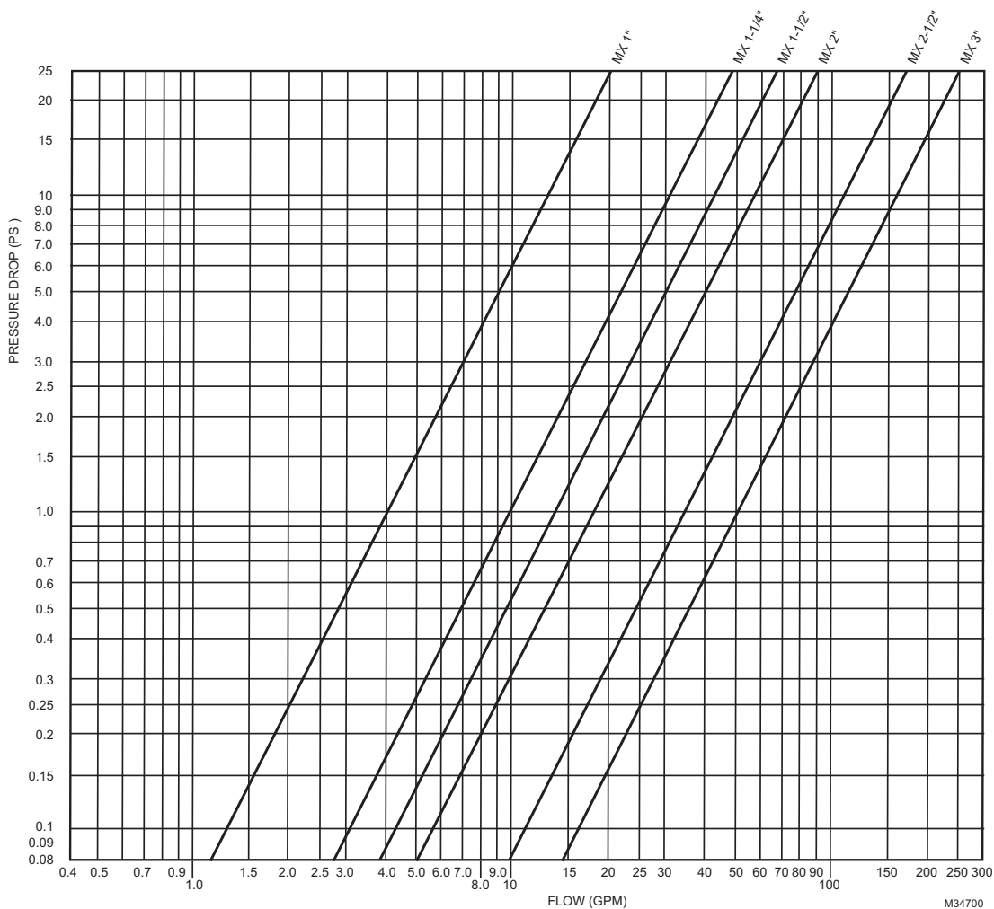
Pressure Drop Chart
