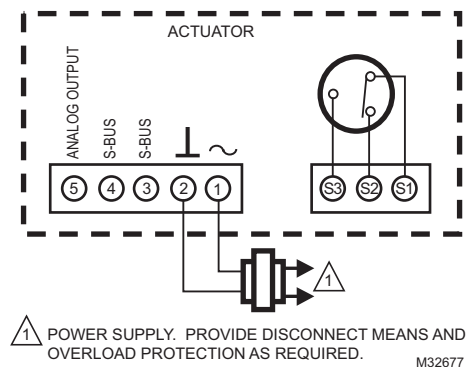
Fig. 11. S-BUS Terminal block details.
