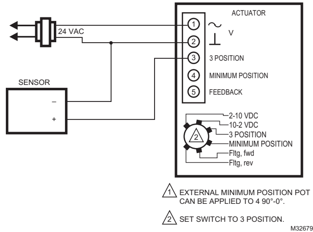
Fig. 20. Wiring for 3 position Economizer controllers, MS74 series.
