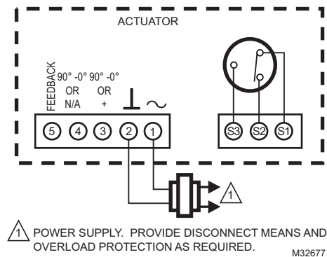
Fig. 10. Terminal block details.
