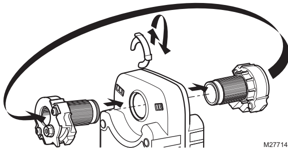
Fig. 3. Mounting shaft coupling to actuator opposite side.
