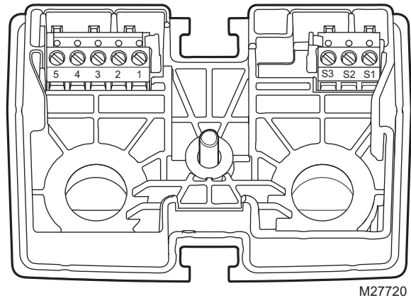
Fig. 9. Terminal block details.
