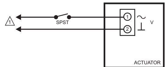
Fig. 12. Wiring for low-voltage two-position control, MS81 series.
