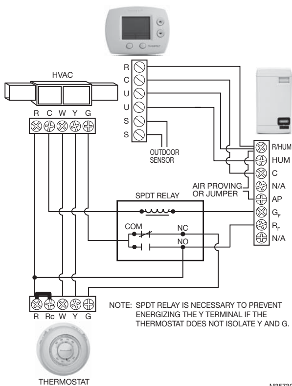
Fig. 18. Wiring the steam humidifier with a mechanical thermostat.
