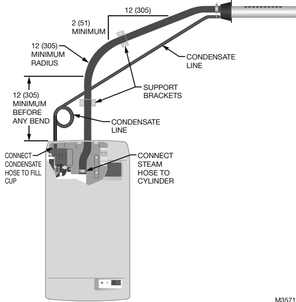
Fig. 12. Steam distributor above humidifier (hose). Measurements in inches (mm).
