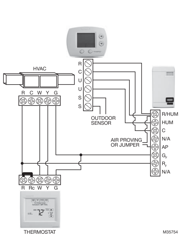
Fig. 17. Wiring the steam humidifier with a digital thermostat.
