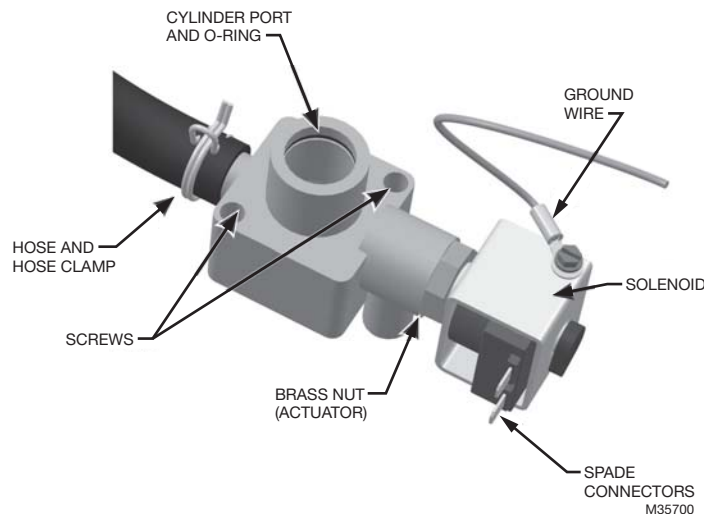
Fig. 1. Drain valve.
