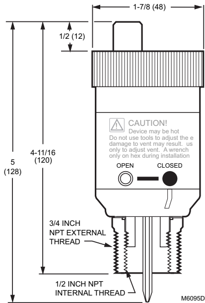
Dimension Diagrams
