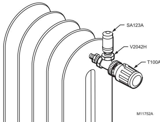
Typical Installation
