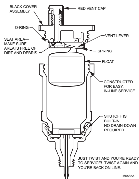
EA122A construction.
