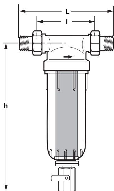
Dimensions Diagram
