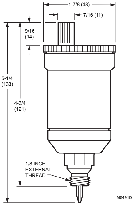
Dimensions Diagram
