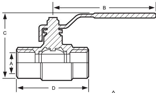
Dimensions Diagram
