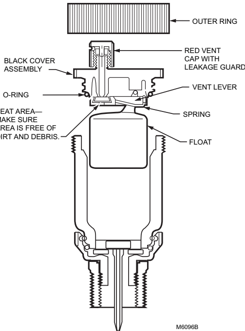
EA79 construction.
