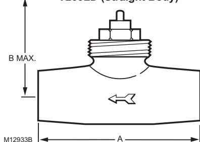
V200LD (Straight Body)
