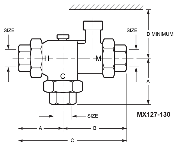
Dimensions Diagram
