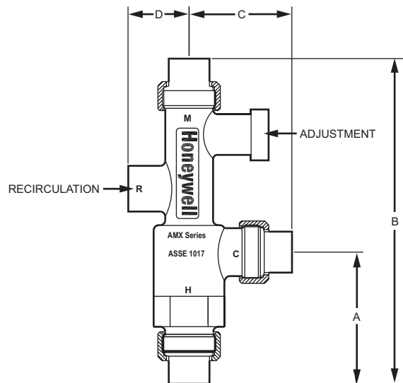
Dimensions Diagram
