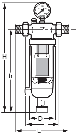
Dimensions Diagram
