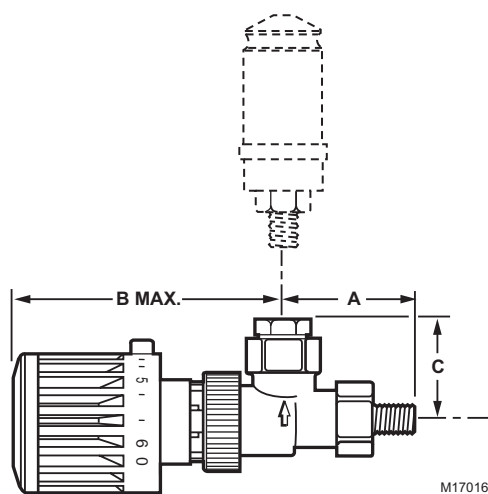
Dimensions Diagram
