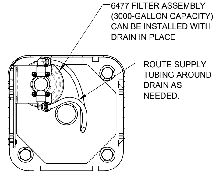
6477 FILTER AND SUPPLY LINE INTERNAL TOP-DOWN PEDESTAL VIEW SCALE 1:8
