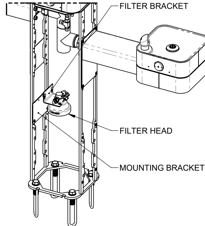
6477 FILTER HEAD/BACKET MOUNTING (ASSEMBLED) (PEDESTAL SIDES, DRAIN HIDDEN FOR CLARITY)
