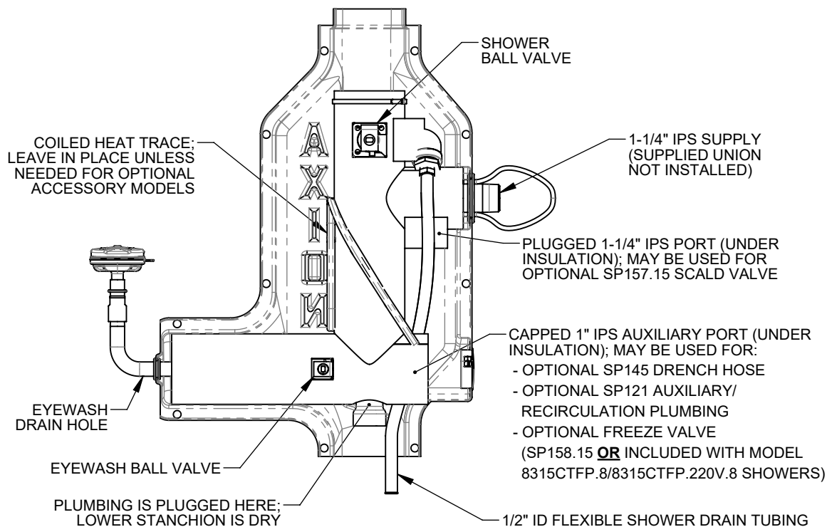
FACTORY-ASSEMBLED SECTION (ZIP TIES HIDDEN FOR CLARITY)
