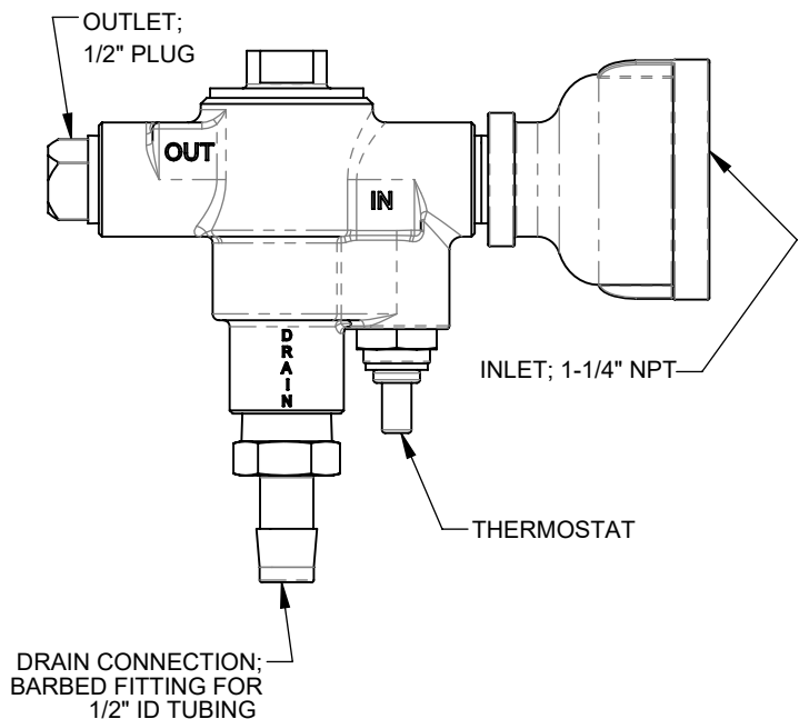
FACTORY-ASSEMBLED VALVE SECTION (8315CTFP.8 & 8315CTFP.220V.8 MODELS ONLY)
